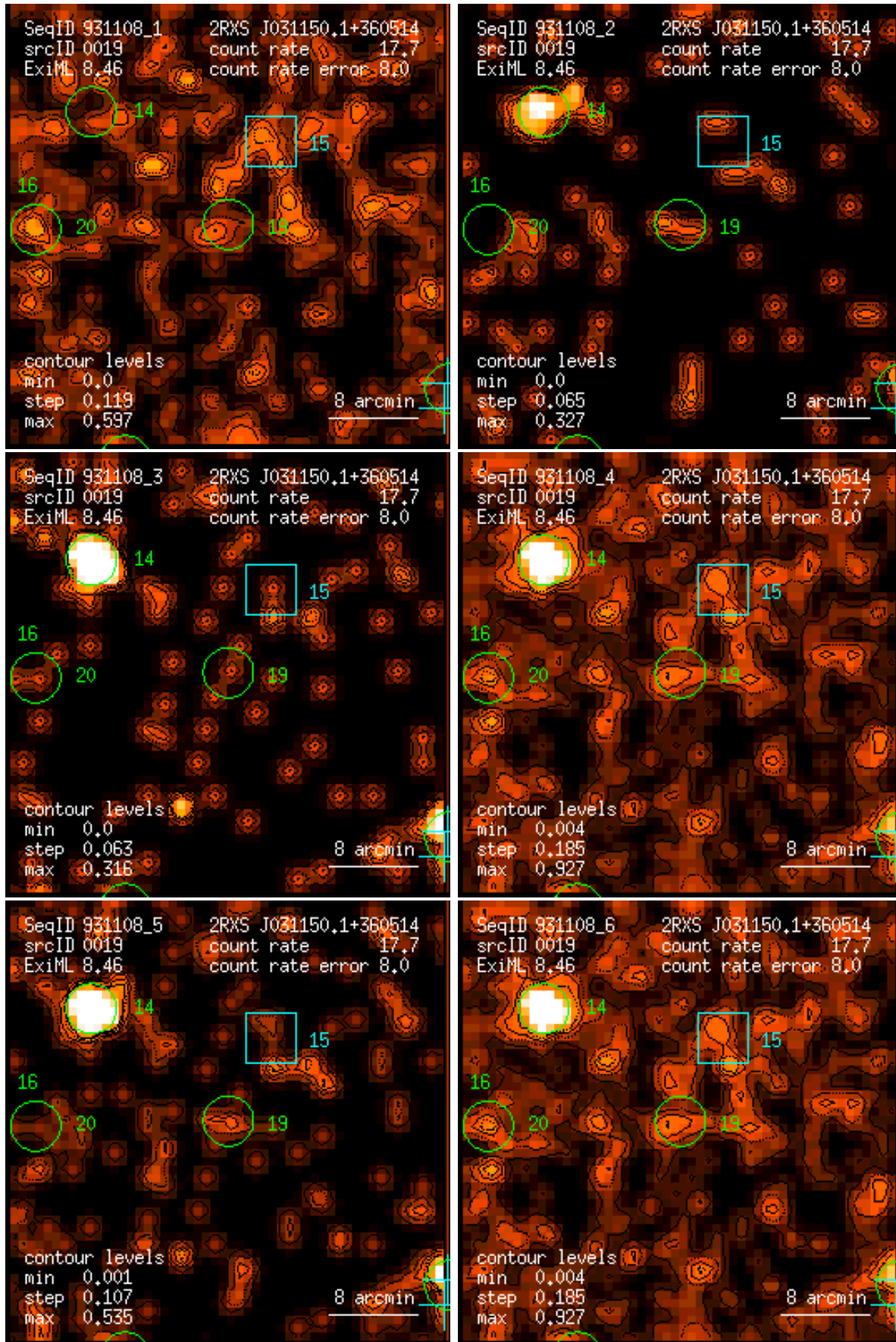
Figure 19: RASS 931108: detection 0019: band rate images, Gaussian filter: (1) PSPC channels 11 – 41, (2) 52 – 90, (3) 91 – 201, (4) 11 – 235, (5) 52 – 201, (6) 11 – 201. Broad band rates in counts/ks. Band rate contour levels in counts/ks/arcmin 2 .
