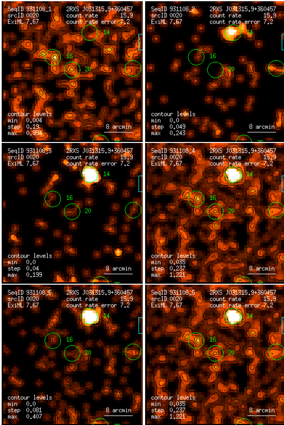
Figure 20: RASS 931108: detection 0020: band rate images, Gaussian filter: (1) PSPC channels 11 – 41, (2) 52 – 90, (3) 91 – 201, (4) 11 – 235, (5) 52 – 201, (6) 11 – 201. Broad band rates in counts/ks. Band rate contour levels in counts/ks/arcmin 2 .
