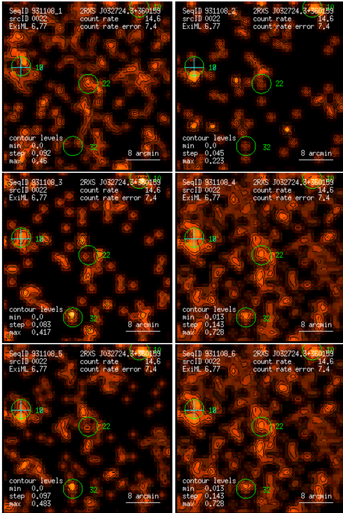
Figure 22: RASS 931108: detection 0022: band rate images, Gaussian filter: (1) PSPC channels 11 – 41, (2) 52 – 90, (3) 91 – 201, (4) 11 – 235, (5) 52 – 201, (6) 11 – 201. Broad band rates in counts/ks. Band rate contour levels in counts/ks/arcmin 2 .
