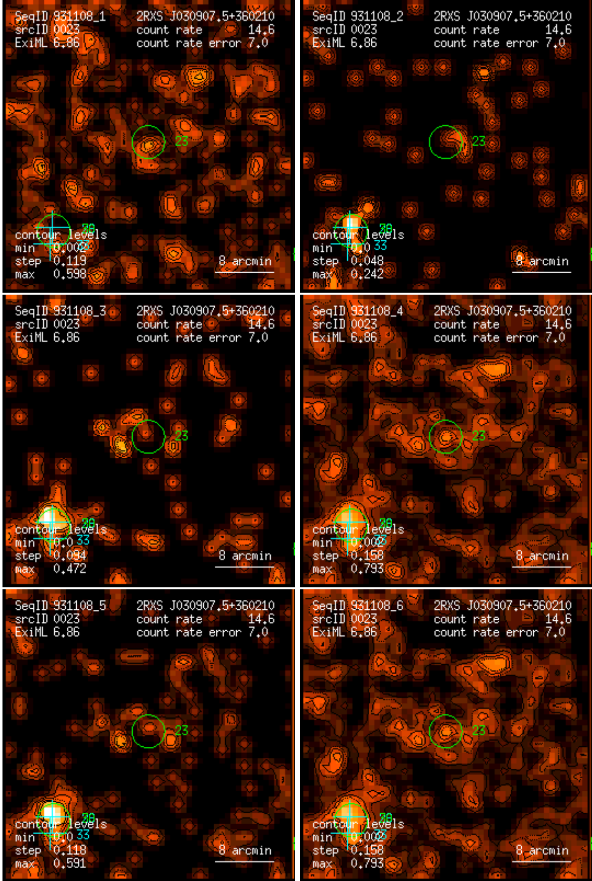
Figure 23: RASS 931108: detection 0023: band rate images, Gaussian filter: (1) PSPC channels 11 – 41, (2) 52 – 90, (3) 91 – 201, (4) 11 – 235, (5) 52 – 201, (6) 11 – 201. Broad band rates in counts/ks. Band rate contour levels in counts/ks/arcmin 2 .
