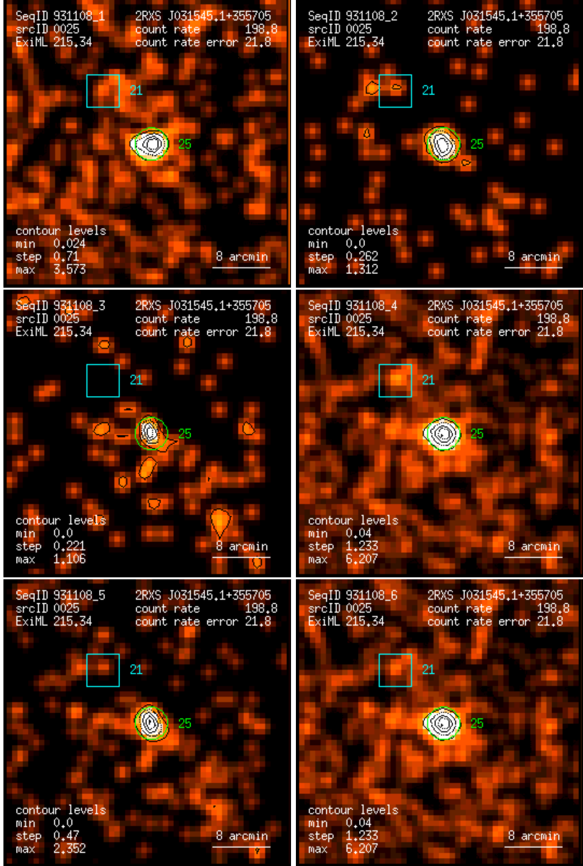
Figure 25: RASS 931108: detection 0025: band rate images, Gaussian filter: (1) PSPC channels 11 – 41, (2) 52 – 90, (3) 91 – 201, (4) 11 – 235, (5) 52 – 201, (6) 11 – 201. Broad band rates in counts/ks. Band rate contour levels in counts/ks/arcmin 2 .
