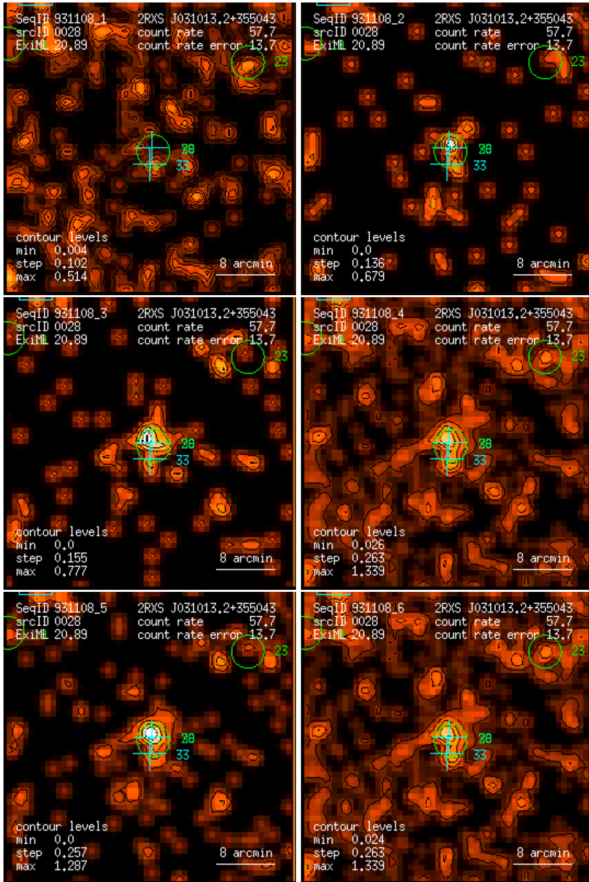
Figure 28: RASS 931108: detection 0028: band rate images, Gaussian filter: (1) PSPC channels 11 – 41, (2) 52 – 90, (3) 91 – 201, (4) 11 – 235, (5) 52 – 201, (6) 11 – 201. Broad band rates in counts/ks. Band rate contour levels in counts/ks/arcmin 2 .
