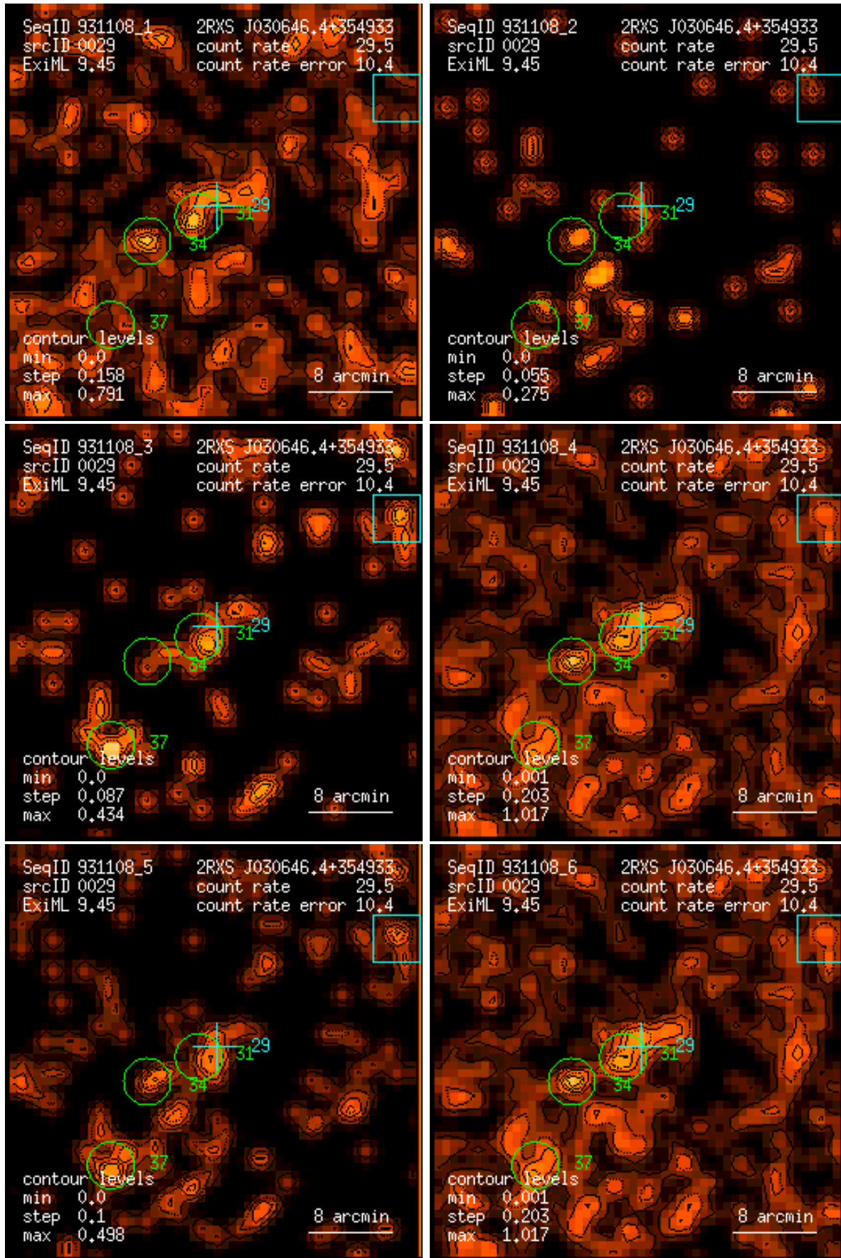
Figure 29: RASS 931108: detection 0029: band rate images, Gaussian filter: (1) PSPC channels 11 – 41, (2) 52 – 90, (3) 91 – 201, (4) 11 – 235, (5) 52 – 201, (6) 11 – 201. Broad band rates in counts/ks. Band rate contour levels in counts/ks/arcmin 2 .
