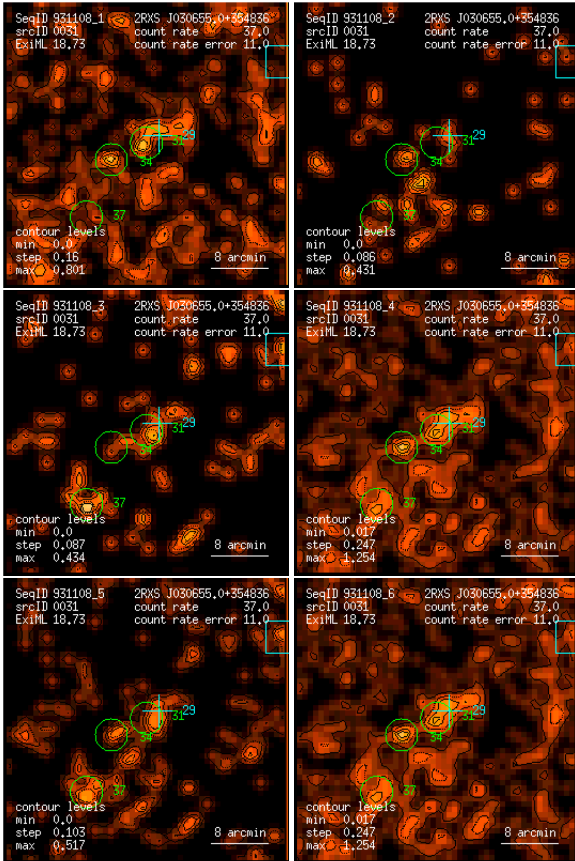
Figure 31: RASS 931108: detection 0031: band rate images, Gaussian filter: (1) PSPC channels 11 – 41, (2) 52 – 90, (3) 91 – 201, (4) 11 – 235, (5) 52 – 201, (6) 11 – 201. Broad band rates in counts/ks. Band rate contour levels in counts/ks/arcmin 2 .
