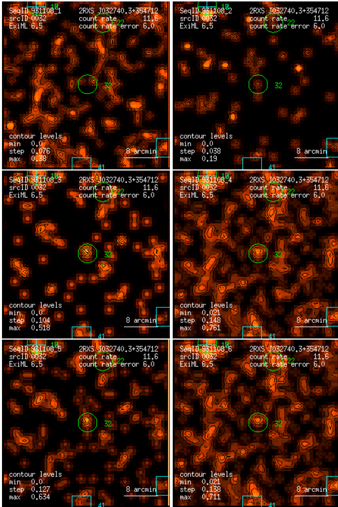
Figure 32: RASS 931108: detection 0032: band rate images, Gaussian filter: (1) PSPC channels 11 – 41, (2) 52 – 90, (3) 91 – 201, (4) 11 – 235, (5) 52 – 201, (6) 11 – 201. Broad band rates in counts/ks. Band rate contour levels in counts/ks/arcmin 2 .
