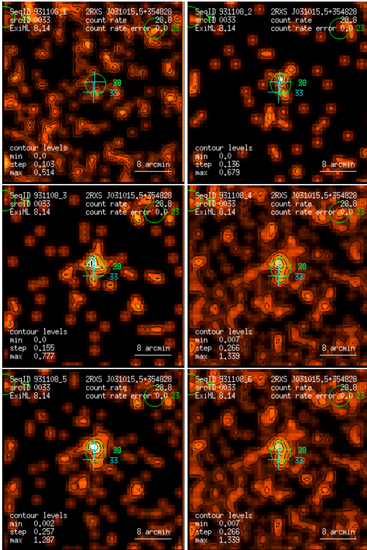
Figure 33: RASS 931108: detection 0033: band rate images, Gaussian filter: (1) PSPC channels 11 – 41, (2) 52 – 90, (3) 91 – 201, (4) 11 – 235, (5) 52 – 201, (6) 11 – 201. Broad band rates in counts/ks. Band rate contour levels in counts/ks/arcmin 2 .
