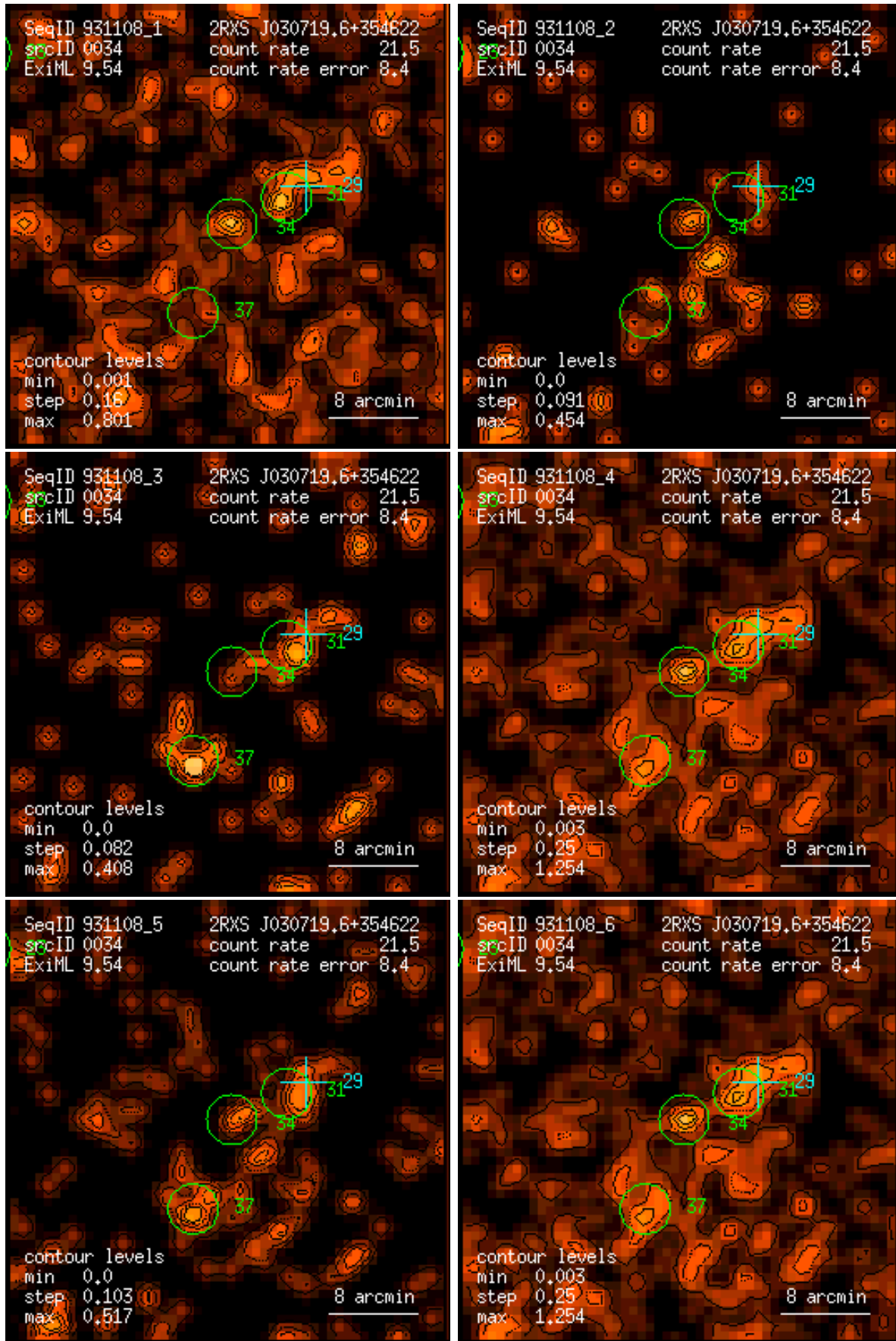
Figure 34: RASS 931108: detection 0034: band rate images, Gaussian filter: (1) PSPC channels 11 – 41, (2) 52 – 90, (3) 91 – 201, (4) 11 – 235, (5) 52 – 201, (6) 11 – 201. Broad band rates in counts/ks. Band rate contour levels in counts/ks/arcmin 2 .
