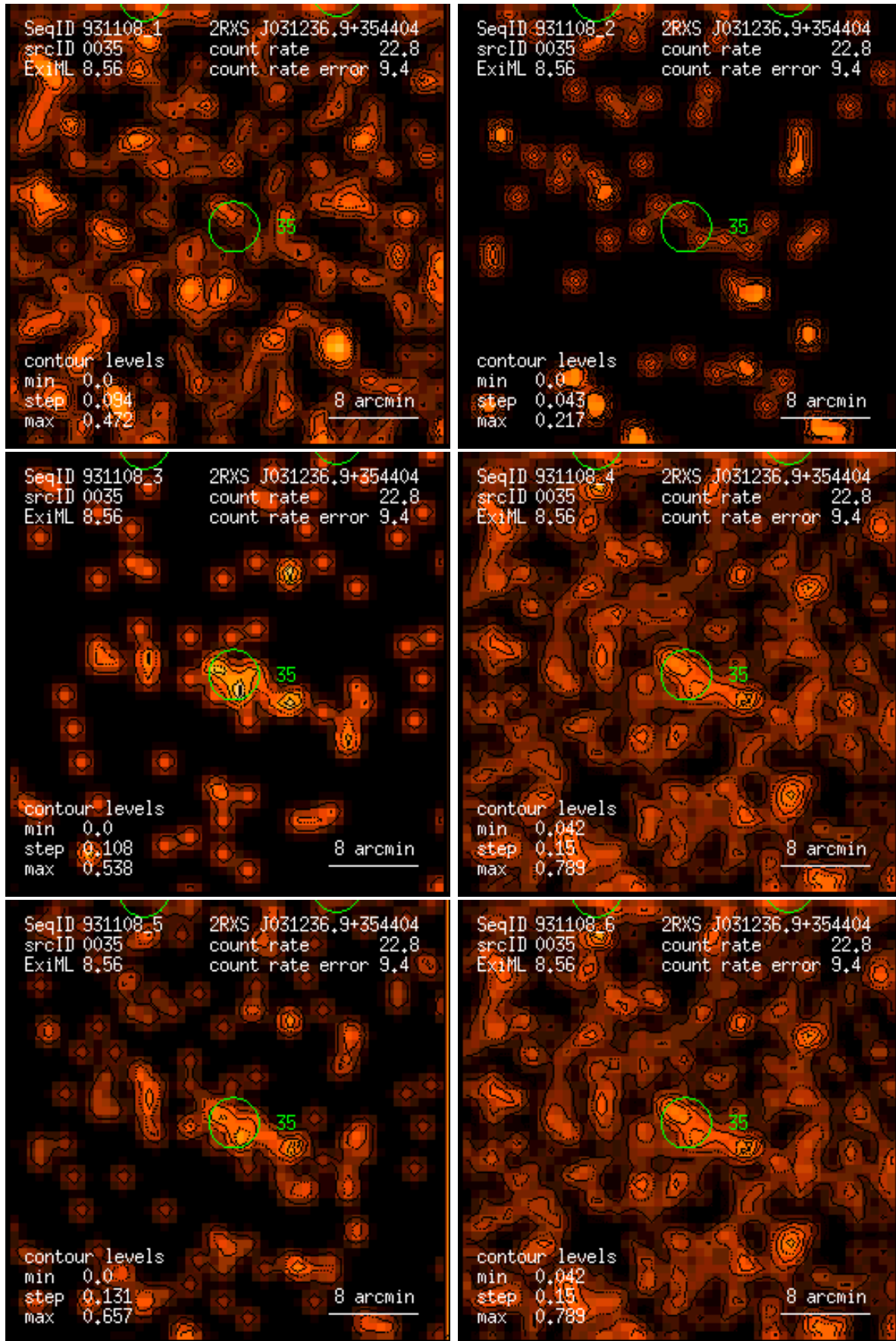
Figure 35: RASS 931108: detection 0035: band rate images, Gaussian filter: (1) PSPC channels 11 – 41, (2) 52 – 90, (3) 91 – 201, (4) 11 – 235, (5) 52 – 201, (6) 11 – 201. Broad band rates in counts/ks. Band rate contour levels in counts/ks/arcmin 2 .
