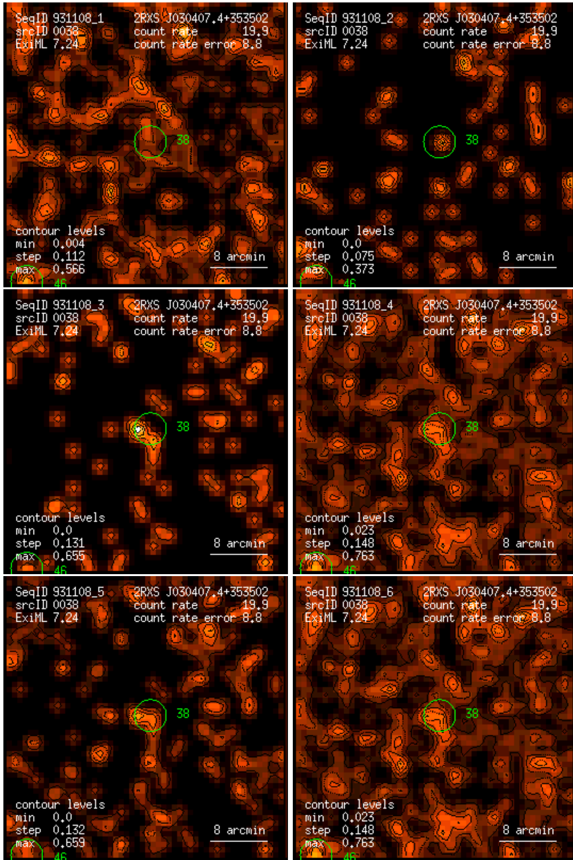
Figure 38: RASS 931108: detection 0038: band rate images, Gaussian filter: (1) PSPC channels 11 – 41, (2) 52 – 90, (3) 91 – 201, (4) 11 – 235, (5) 52 – 201, (6) 11 – 201. Broad band rates in counts/ks. Band rate contour levels in counts/ks/arcmin 2 .
