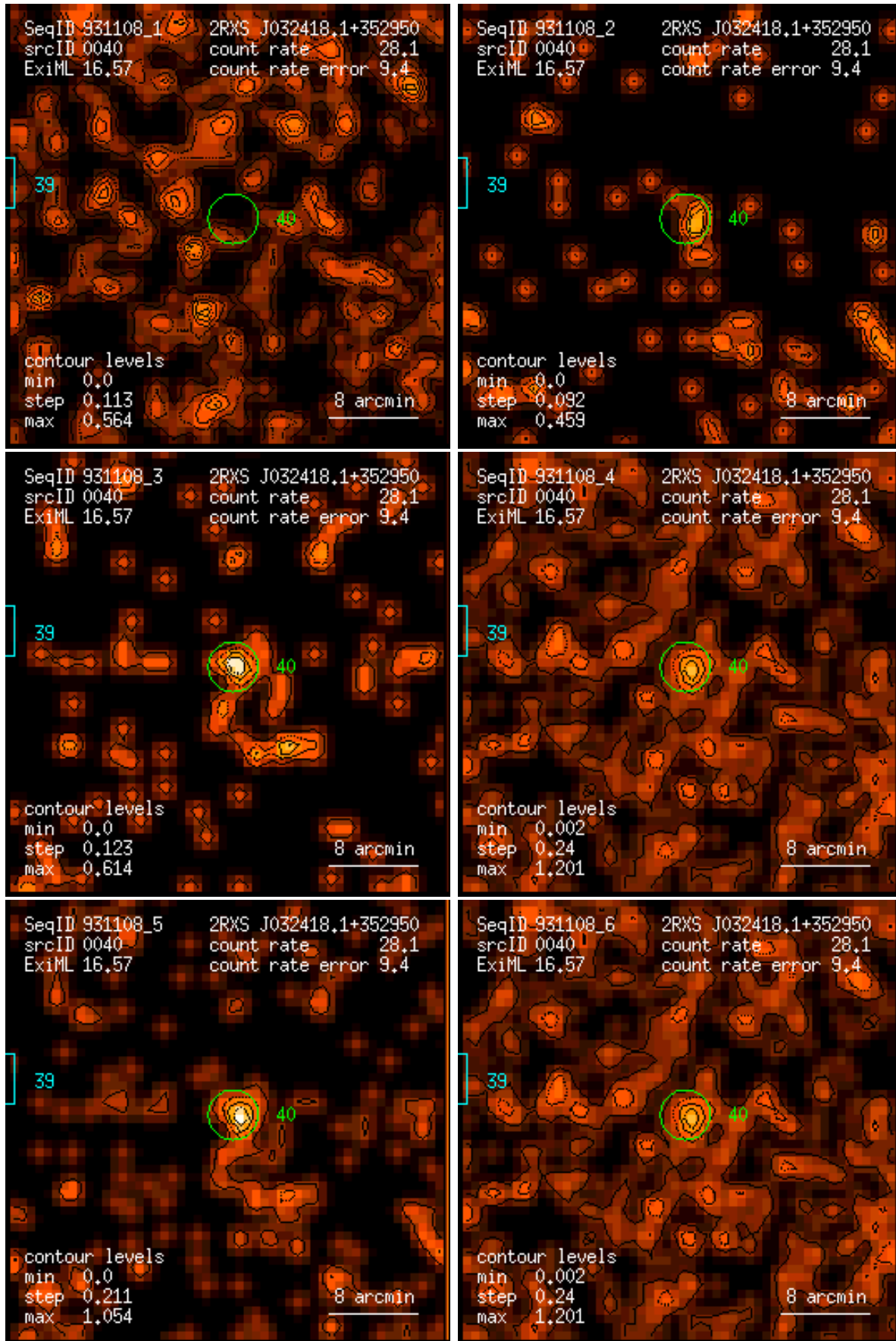
Figure 40: RASS 931108: detection 0040: band rate images, Gaussian filter: (1) PSPC channels 11 – 41, (2) 52 – 90, (3) 91 – 201, (4) 11 – 235, (5) 52 – 201, (6) 11 – 201. Broad band rates in counts/ks. Band rate contour levels in counts/ks/arcmin 2 .
