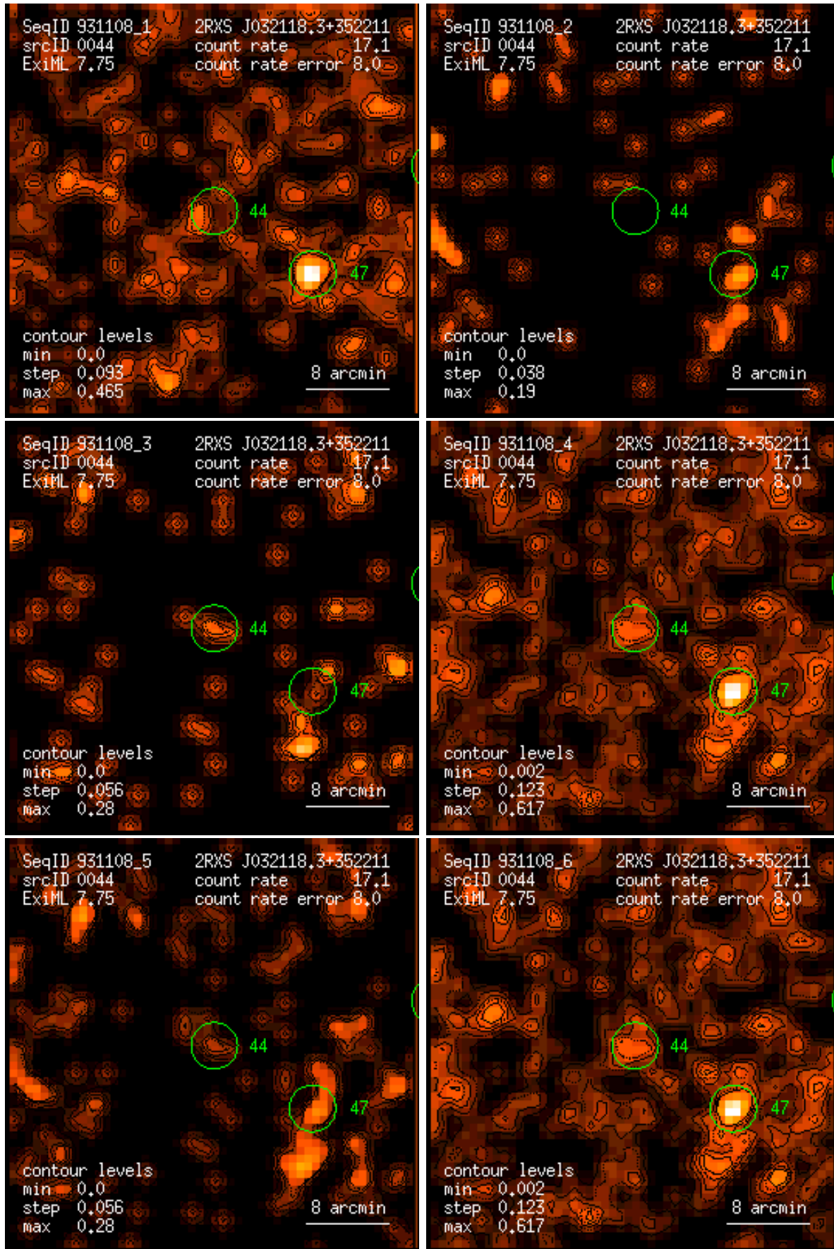
Figure 44: RASS 931108: detection 0044: band rate images, Gaussian filter: (1) PSPC channels 11 – 41, (2) 52 – 90, (3) 91 – 201, (4) 11 – 235, (5) 52 – 201, (6) 11 – 201. Broad band rates in counts/ks. Band rate contour levels in counts/ks/arcmin 2 .
