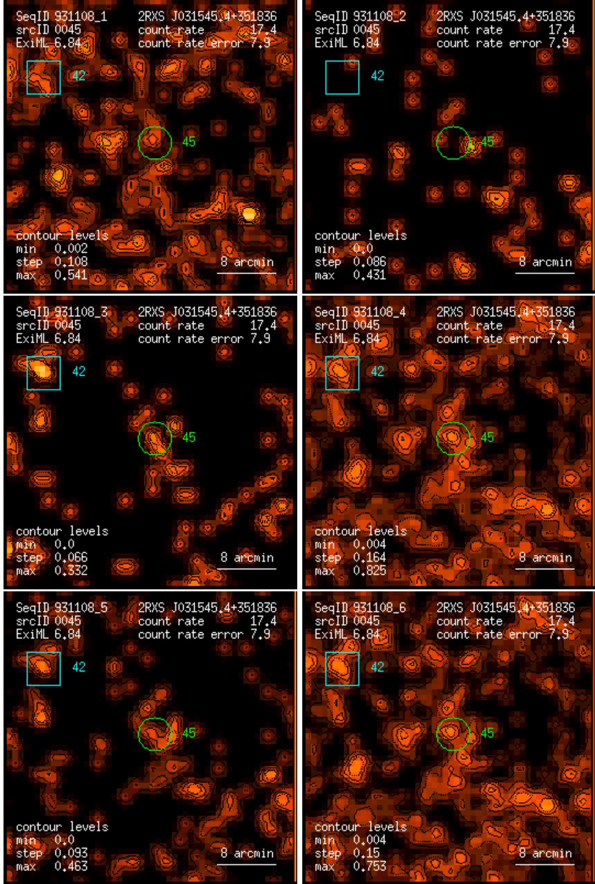
Figure 45: RASS 931108: detection 0045: band rate images, Gaussian filter: (1) PSPC channels 11 – 41, (2) 52 – 90, (3) 91 – 201, (4) 11 – 235, (5) 52 – 201, (6) 11 – 201. Broad band rates in counts/ks. Band rate contour levels in counts/ks/arcmin 2 .
