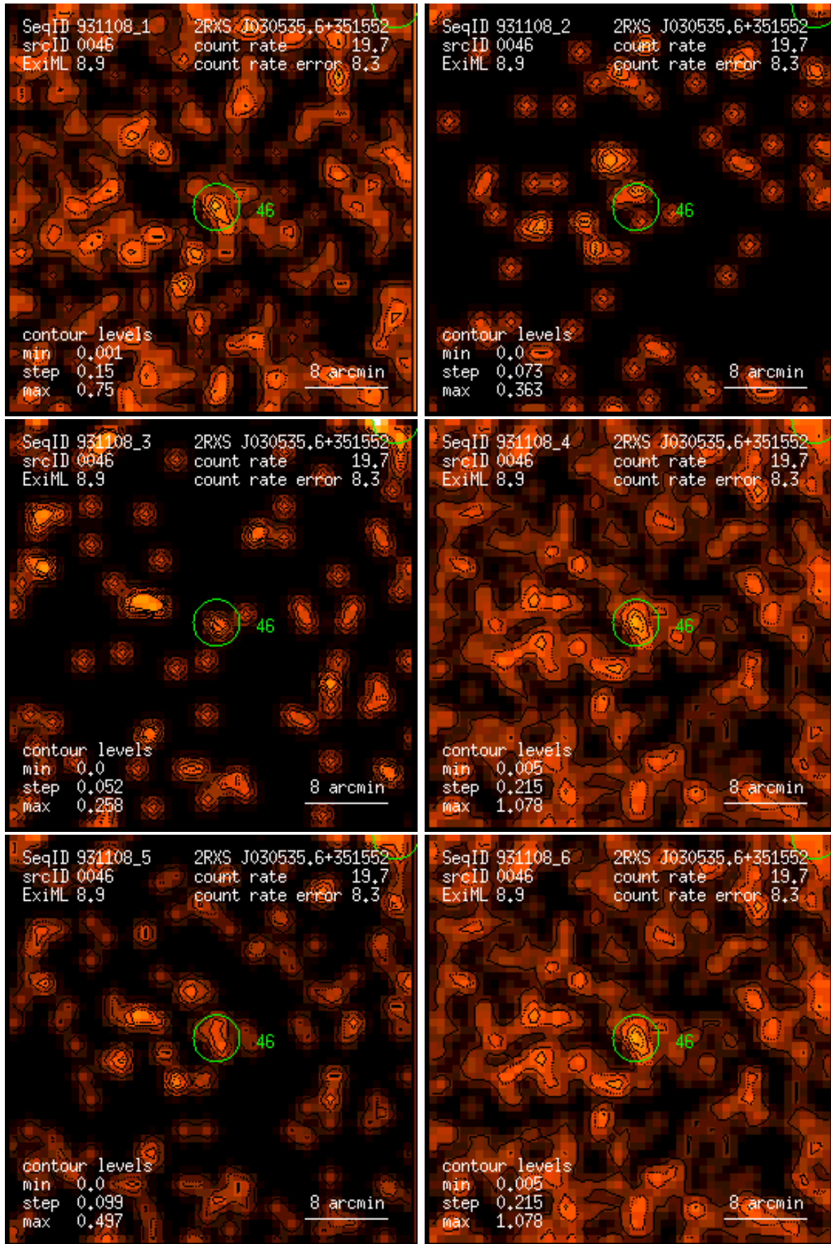
Figure 46: RASS 931108: detection 0046: band rate images, Gaussian filter: (1) PSPC channels 11 – 41, (2) 52 – 90, (3) 91 – 201, (4) 11 – 235, (5) 52 – 201, (6) 11 – 201. Broad band rates in counts/ks. Band rate contour levels in counts/ks/arcmin 2 .
