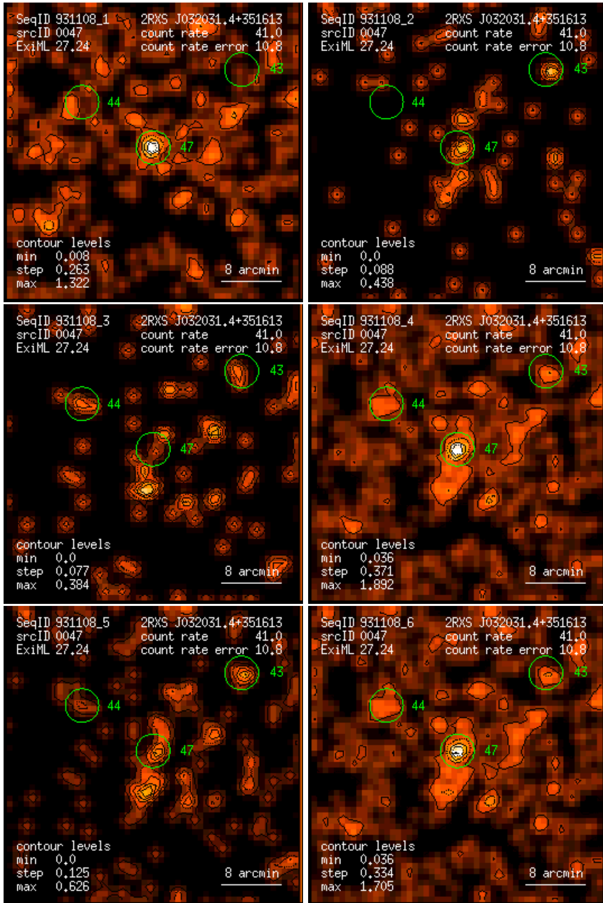
Figure 47: RASS 931108: detection 0047: band rate images, Gaussian filter: (1) PSPC channels 11 – 41, (2) 52 – 90, (3) 91 – 201, (4) 11 – 235, (5) 52 – 201, (6) 11 – 201. Broad band rates in counts/ks. Band rate contour levels in counts/ks/arcmin 2 .
