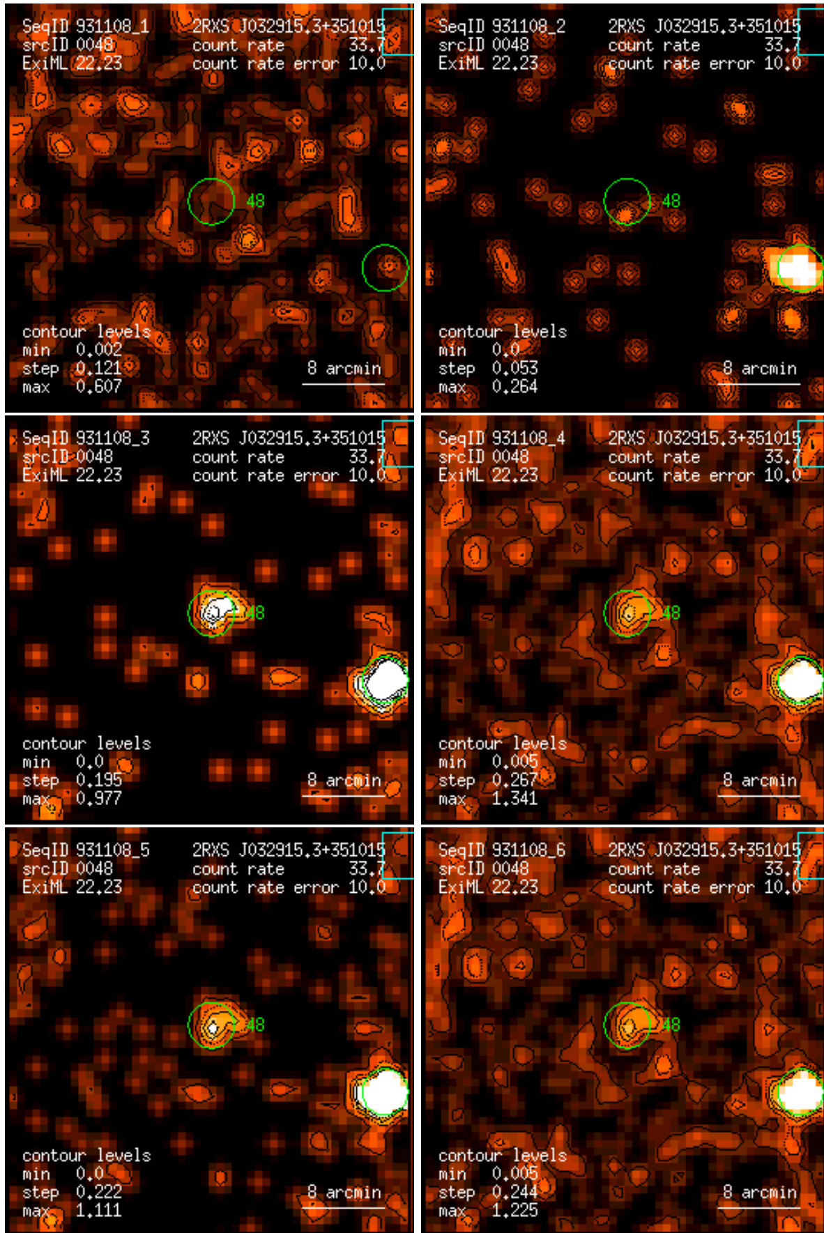
Figure 48: RASS 931108: detection 0048: band rate images, Gaussian filter: (1) PSPC channels 11 – 41, (2) 52 – 90, (3) 91 – 201, (4) 11 – 235, (5) 52 – 201, (6) 11 – 201. Broad band rates in counts/ks. Band rate contour levels in counts/ks/arcmin 2 .
