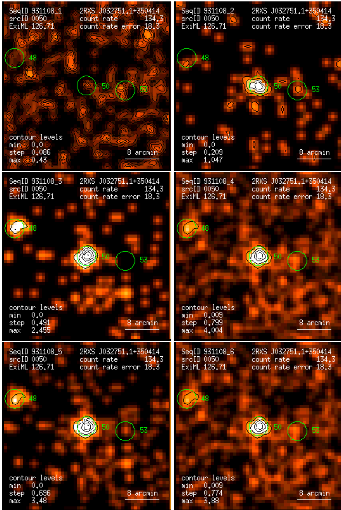
Figure 50: RASS 931108: detection 0050: band rate images, Gaussian filter: (1) PSPC channels 11 – 41, (2) 52 – 90, (3) 91 – 201, (4) 11 – 235, (5) 52 – 201, (6) 11 – 201. Broad band rates in counts/ks. Band rate contour levels in counts/ks/arcmin 2 .
