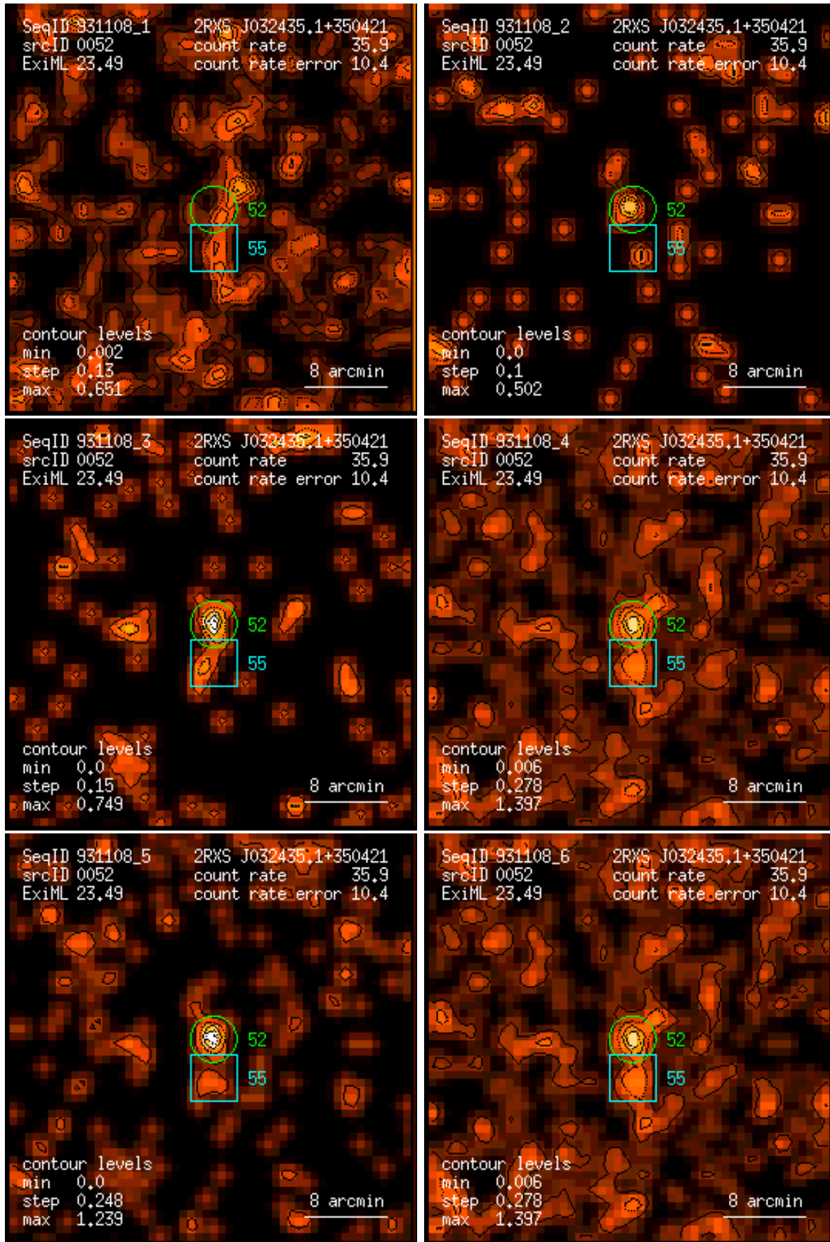
Figure 52: RASS 931108: detection 0052: band rate images, Gaussian filter: (1) PSPC channels 11 – 41, (2) 52 – 90, (3) 91 – 201, (4) 11 – 235, (5) 52 – 201, (6) 11 – 201. Broad band rates in counts/ks. Band rate contour levels in counts/ks/arcmin 2 .
