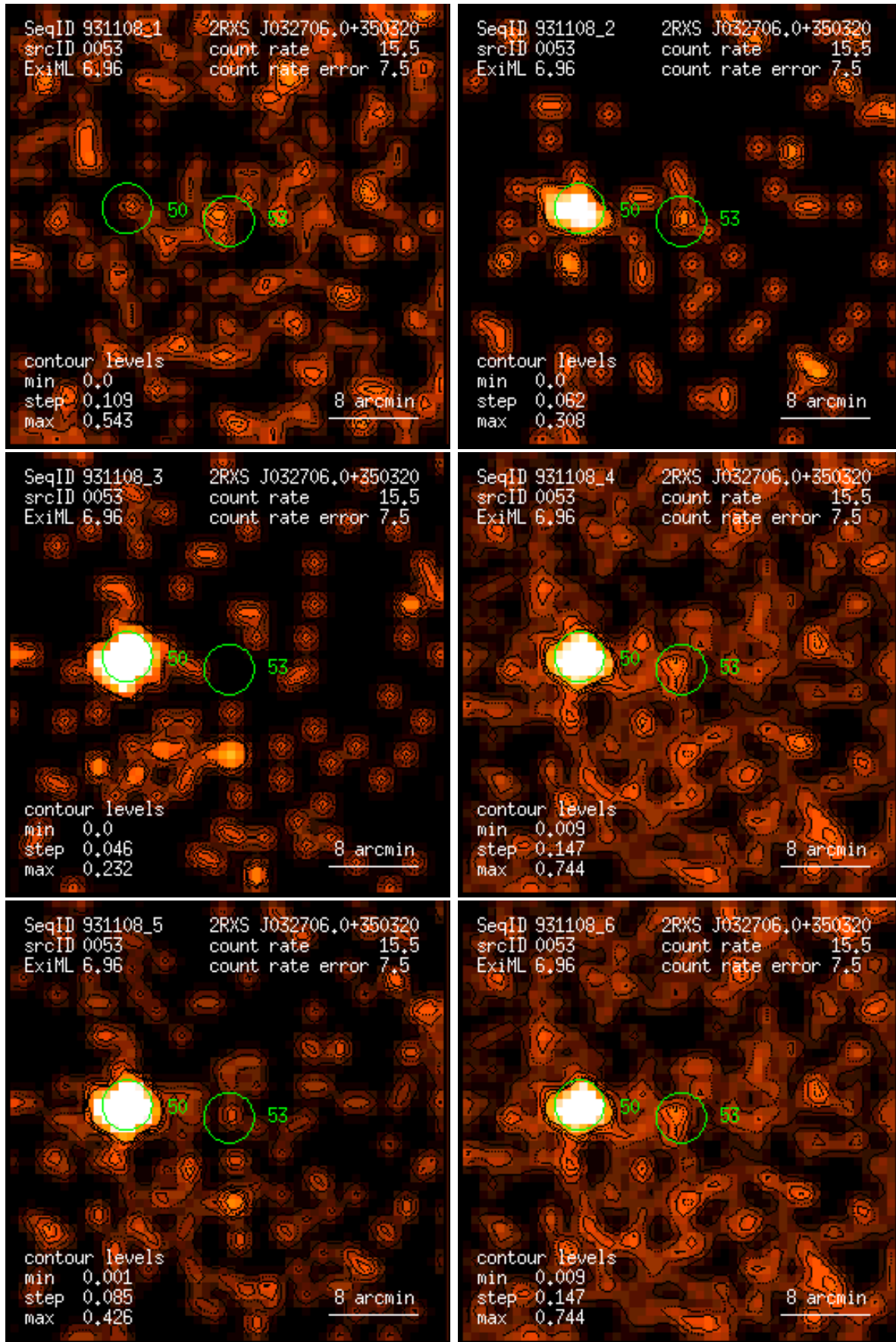
Figure 53: RASS 931108: detection 0053: band rate images, Gaussian filter: (1) PSPC channels 11 – 41, (2) 52 – 90, (3) 91 – 201, (4) 11 – 235, (5) 52 – 201, (6) 11 – 201. Broad band rates in counts/ks. Band rate contour levels in counts/ks/arcmin 2 .
