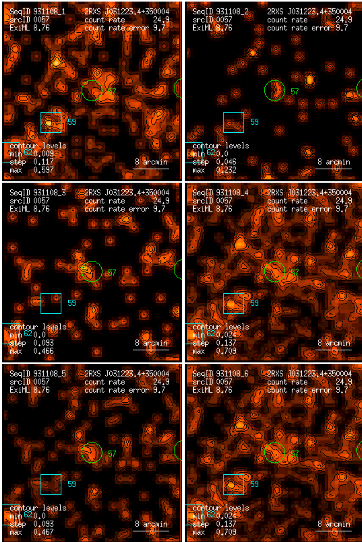
Figure 57: RASS 931108: detection 0057: band rate images, Gaussian filter: (1) PSPC channels 11 – 41, (2) 52 – 90, (3) 91 – 201, (4) 11 – 235, (5) 52 – 201, (6) 11 – 201. Broad band rates in counts/ks. Band rate contour levels in counts/ks/arcmin 2 .
