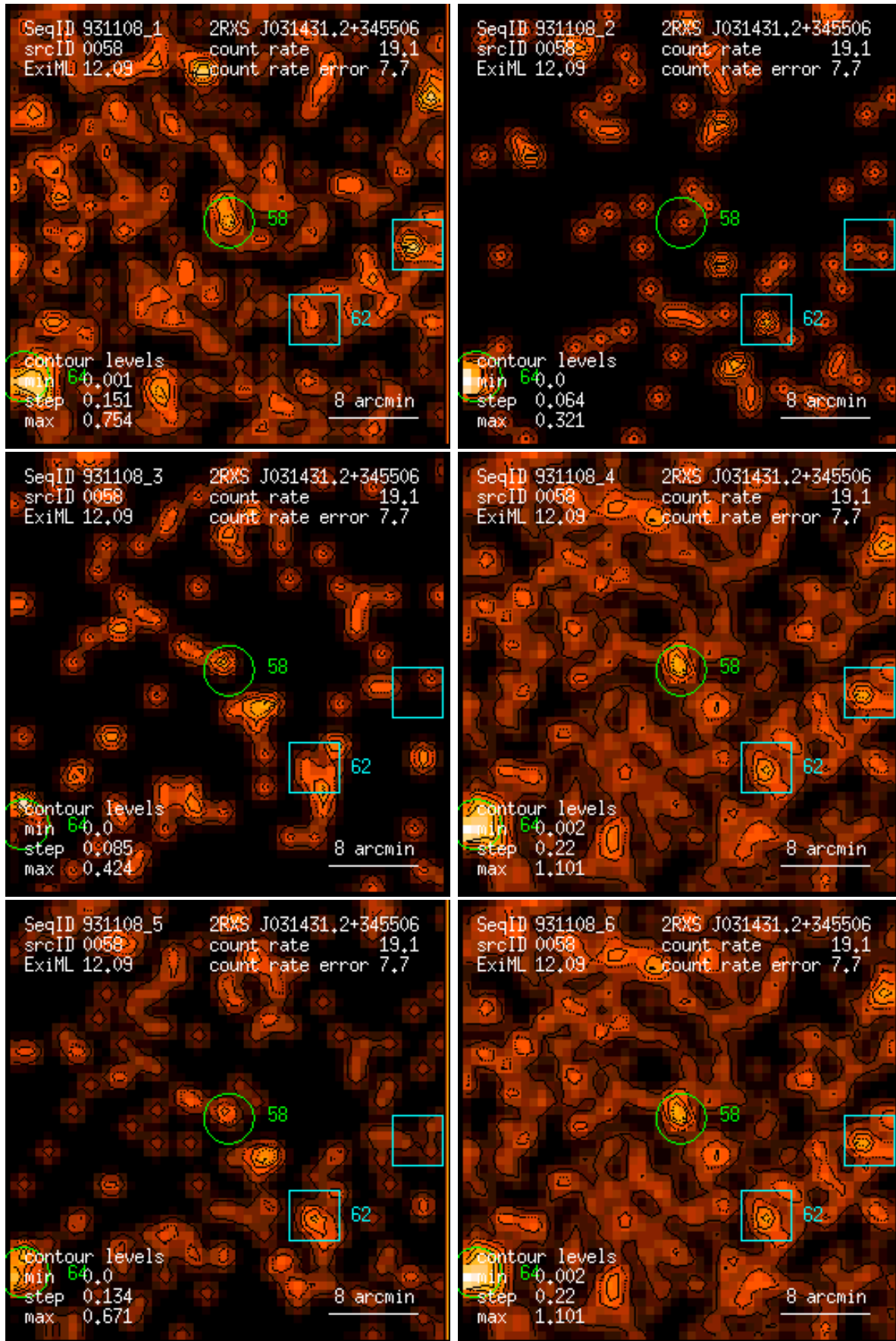
Figure 58: RASS 931108: detection 0058: band rate images, Gaussian filter: (1) PSPC channels 11 – 41, (2) 52 – 90, (3) 91 – 201, (4) 11 – 235, (5) 52 – 201, (6) 11 – 201. Broad band rates in counts/ks. Band rate contour levels in counts/ks/arcmin 2 .
