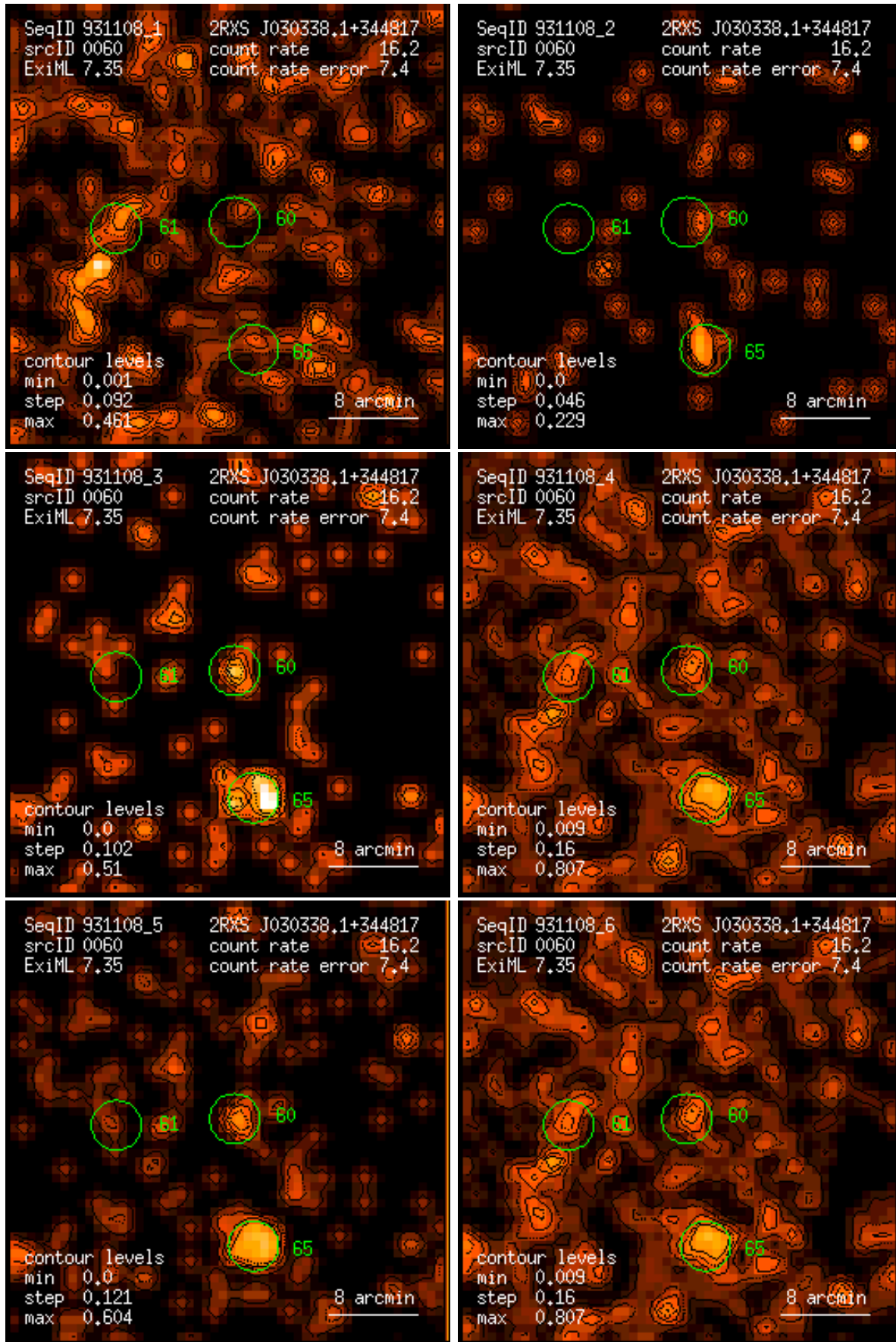
Figure 60: RASS 931108: detection 0060: band rate images, Gaussian filter: (1) PSPC channels 11 – 41, (2) 52 – 90, (3) 91 – 201, (4) 11 – 235, (5) 52 – 201, (6) 11 – 201. Broad band rates in counts/ks. Band rate contour levels in counts/ks/arcmin 2 .
