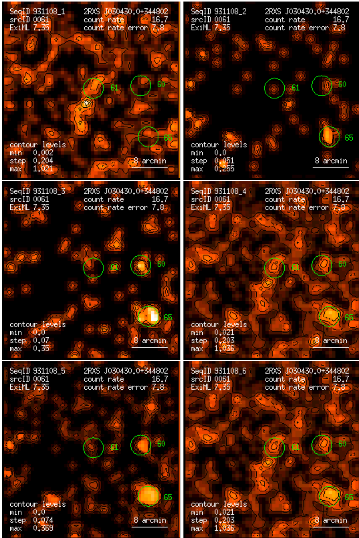
Figure 61: RASS 931108: detection 0061: band rate images, Gaussian filter: (1) PSPC channels 11 – 41, (2) 52 – 90, (3) 91 – 201, (4) 11 – 235, (5) 52 – 201, (6) 11 – 201. Broad band rates in counts/ks. Band rate contour levels in counts/ks/arcmin 2 .
