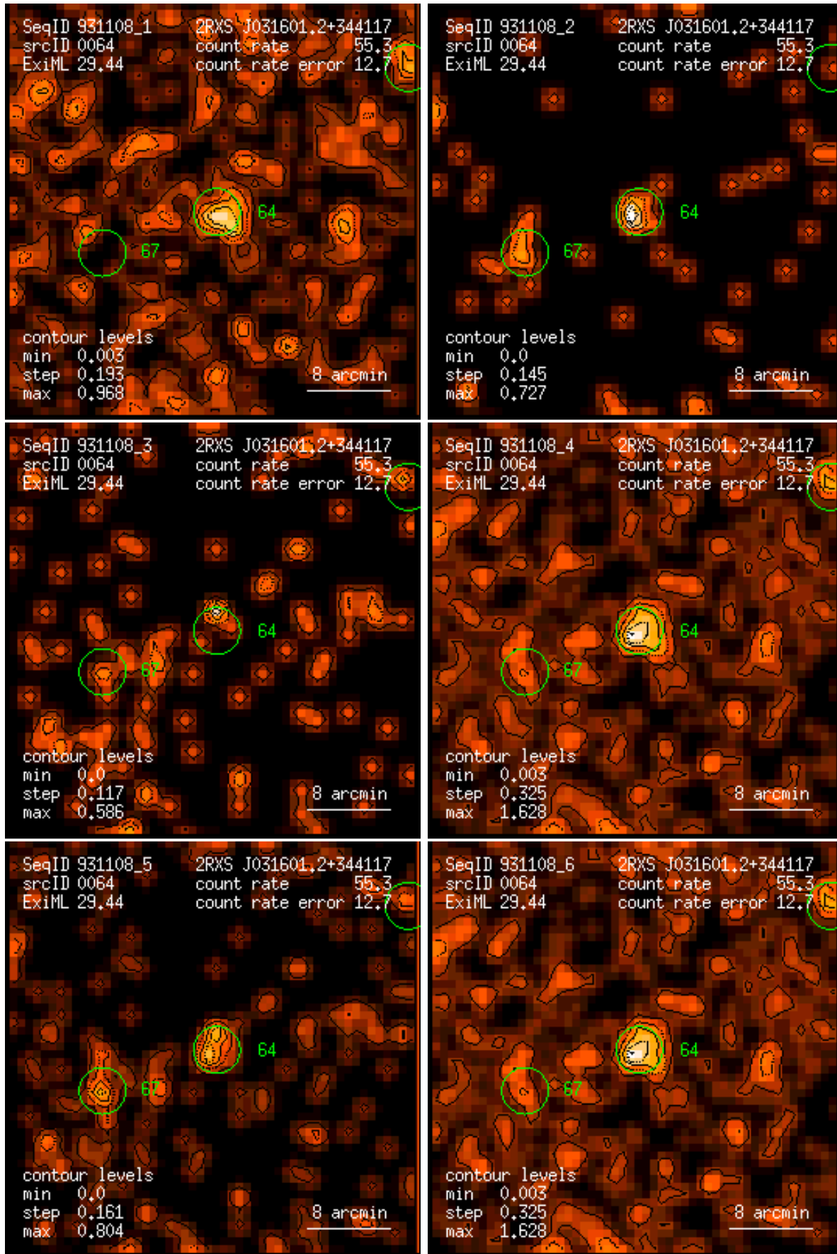
Figure 64: RASS 931108: detection 0064: band rate images, Gaussian filter: (1) PSPC channels 11 – 41, (2) 52 – 90, (3) 91 – 201, (4) 11 – 235, (5) 52 – 201, (6) 11 – 201. Broad band rates in counts/ks. Band rate contour levels in counts/ks/arcmin 2 .
