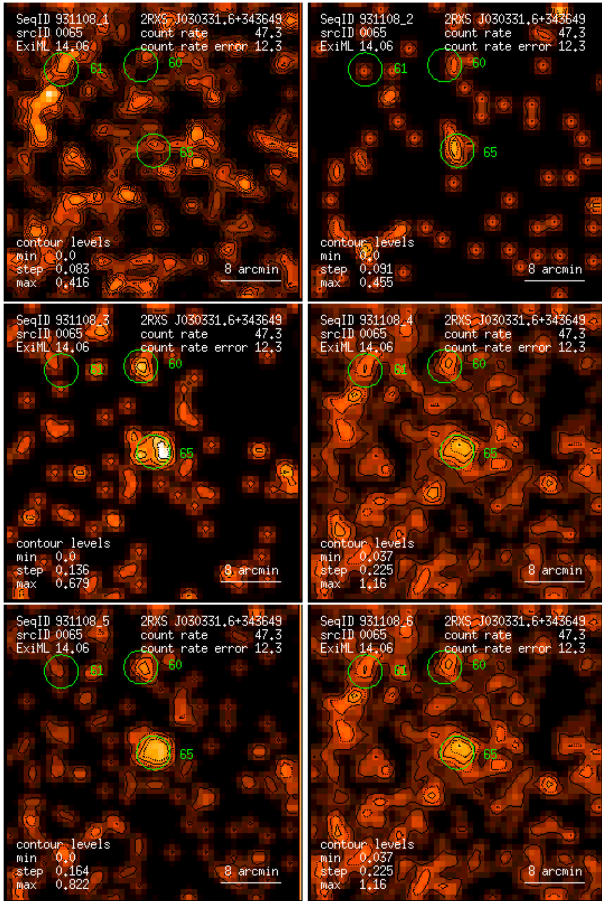
Figure 65: RASS 931108: detection 0065: band rate images, Gaussian filter: (1) PSPC channels 11 – 41, (2) 52 – 90, (3) 91 – 201, (4) 11 – 235, (5) 52 – 201, (6) 11 – 201. Broad band rates in counts/ks. Band rate contour levels in counts/ks/arcmin 2 .
