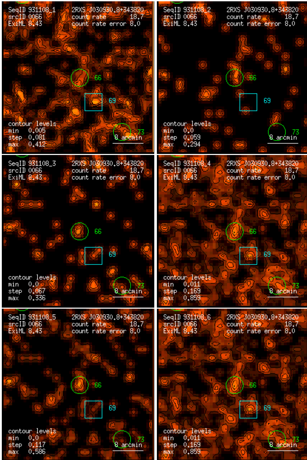
Figure 66: RASS 931108: detection 0066: band rate images, Gaussian filter: (1) PSPC channels 11 – 41, (2) 52 – 90, (3) 91 – 201, (4) 11 – 235, (5) 52 – 201, (6) 11 – 201. Broad band rates in counts/ks. Band rate contour levels in counts/ks/arcmin 2 .
