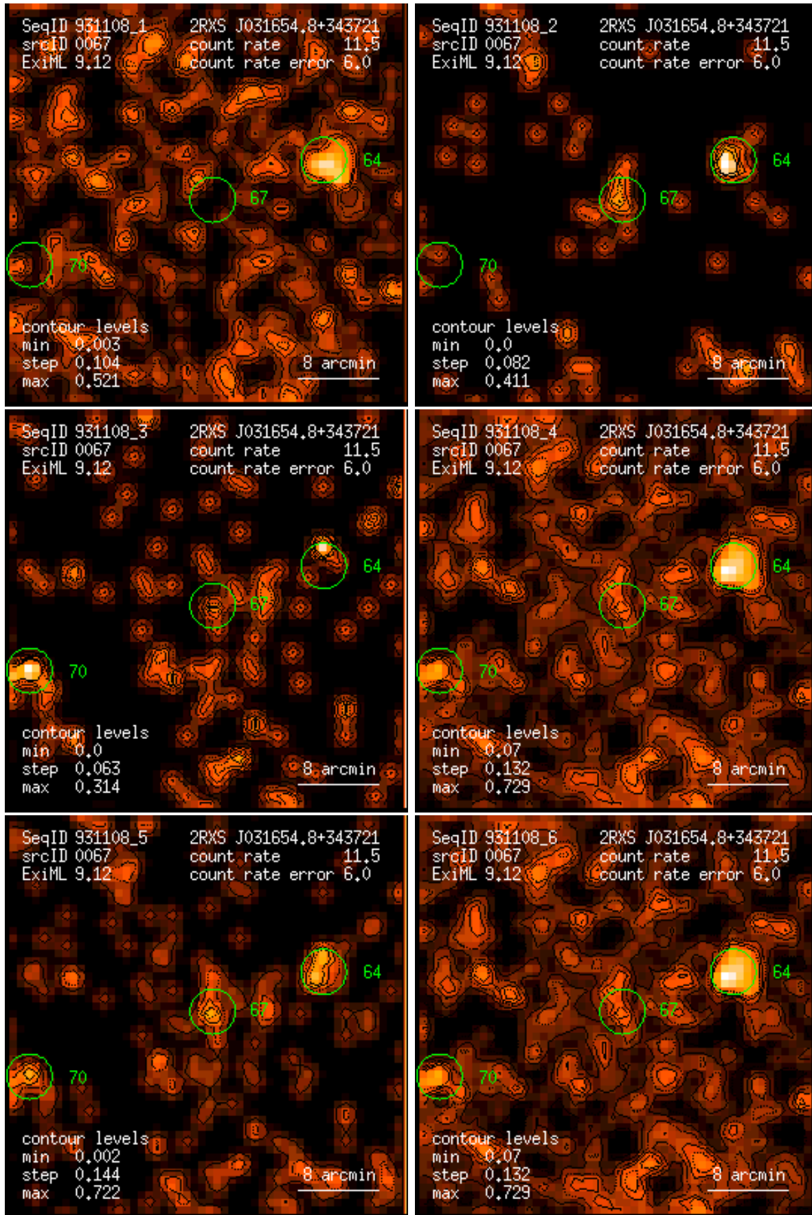
Figure 67: RASS 931108: detection 0067: band rate images, Gaussian filter: (1) PSPC channels 11 – 41, (2) 52 – 90, (3) 91 – 201, (4) 11 – 235, (5) 52 – 201, (6) 11 – 201. Broad band rates in counts/ks. Band rate contour levels in counts/ks/arcmin 2 .
