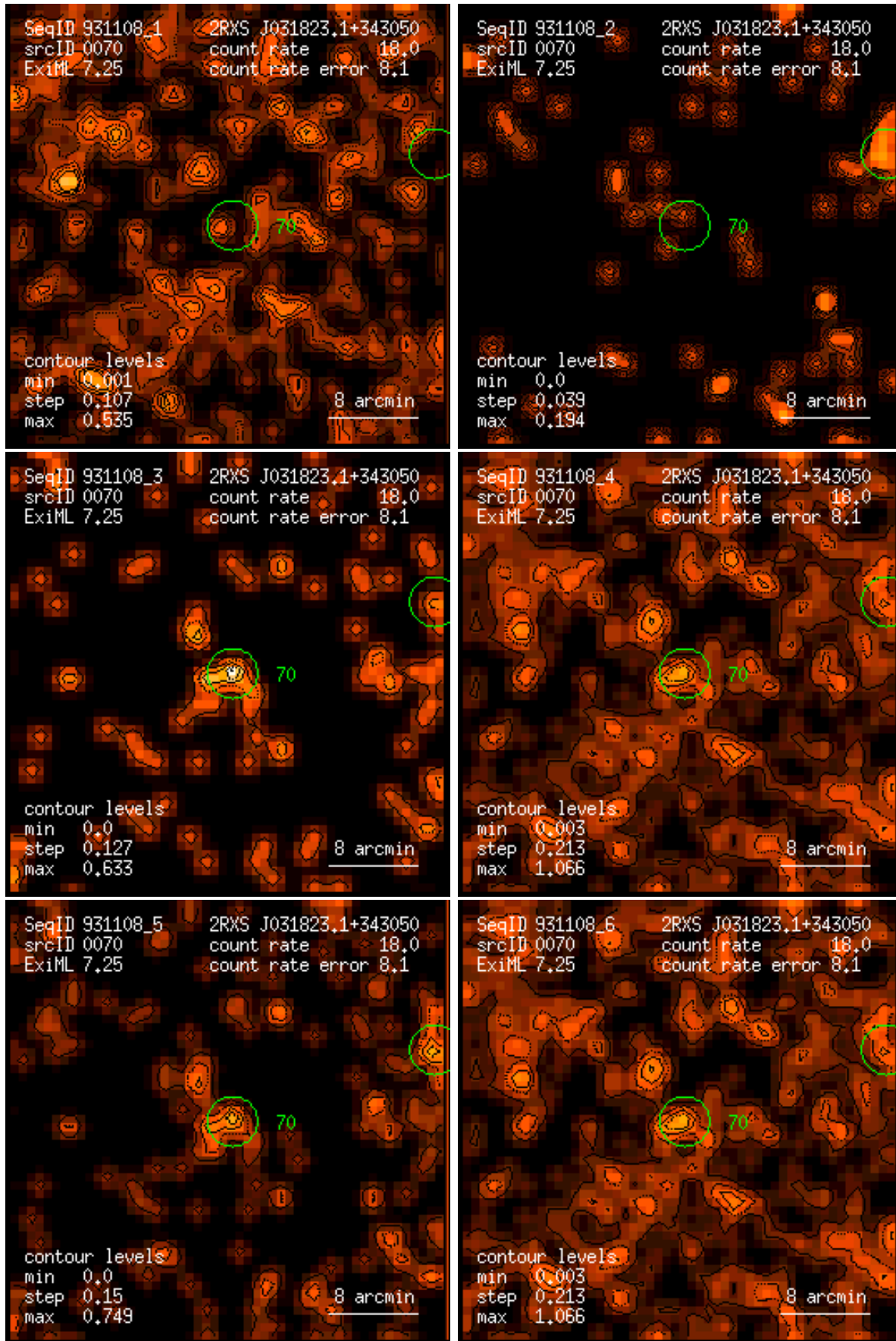
Figure 70: RASS 931108: detection 0070: band rate images, Gaussian filter: (1) PSPC channels 11 – 41, (2) 52 – 90, (3) 91 – 201, (4) 11 – 235, (5) 52 – 201, (6) 11 – 201. Broad band rates in counts/ks. Band rate contour levels in counts/ks/arcmin 2 .
