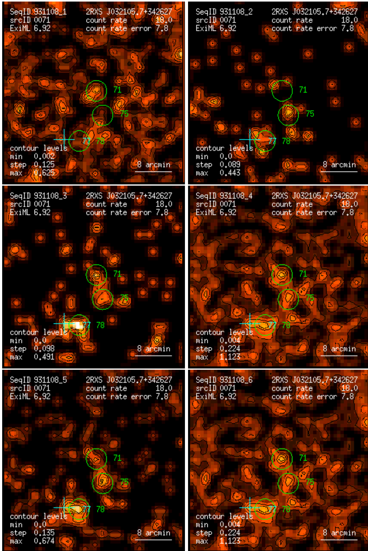
Figure 71: RASS 931108: detection 0071: band rate images, Gaussian filter: (1) PSPC channels 11 – 41, (2) 52 – 90, (3) 91 – 201, (4) 11 – 235, (5) 52 – 201, (6) 11 – 201. Broad band rates in counts/ks. Band rate contour levels in counts/ks/arcmin 2 .
