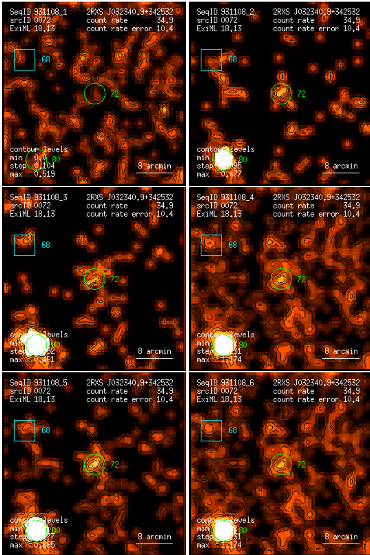
Figure 72: RASS 931108: detection 0072: band rate images, Gaussian filter: (1) PSPC channels 11 – 41, (2) 52 – 90, (3) 91 – 201, (4) 11 – 235, (5) 52 – 201, (6) 11 – 201. Broad band rates in counts/ks. Band rate contour levels in counts/ks/arcmin 2 .
