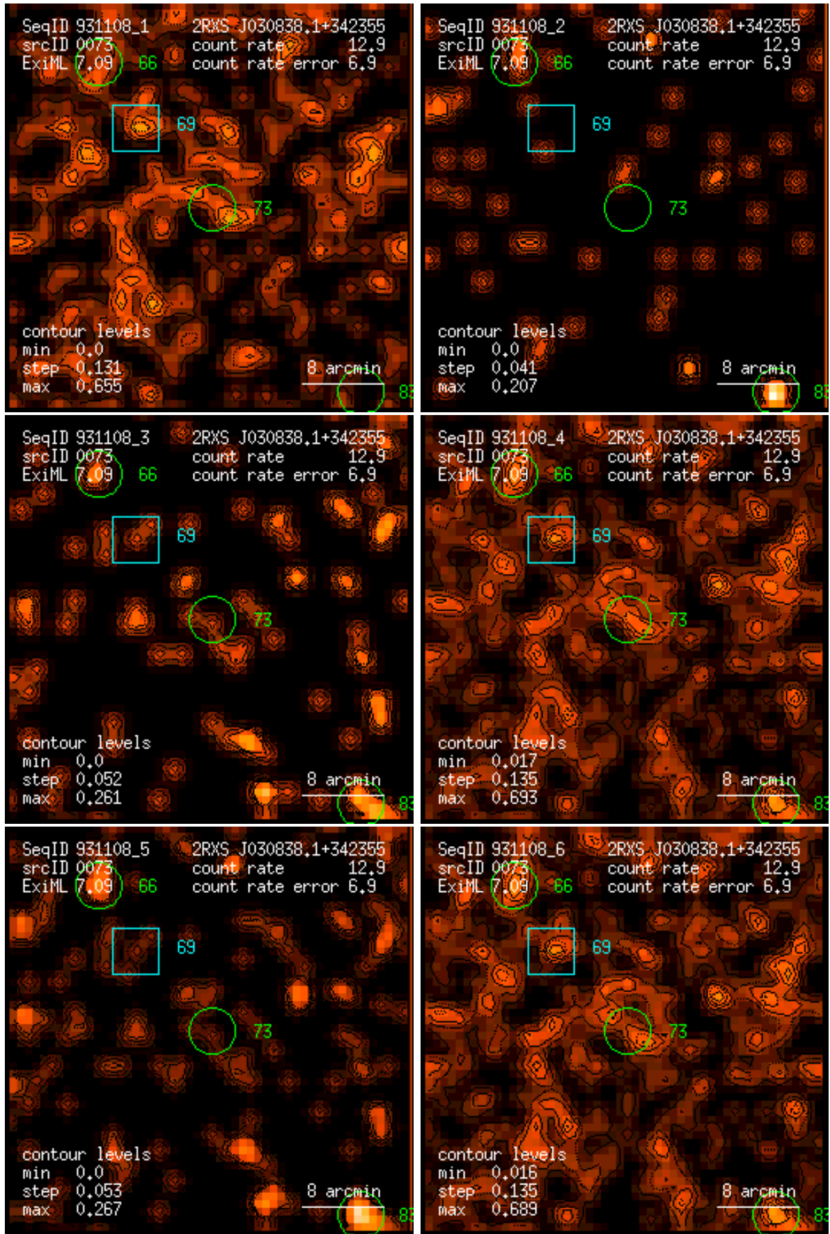
Figure 73: RASS 931108: detection 0073: band rate images, Gaussian filter: (1) PSPC channels 11 – 41, (2) 52 – 90, (3) 91 – 201, (4) 11 – 235, (5) 52 – 201, (6) 11 – 201. Broad band rates in counts/ks. Band rate contour levels in counts/ks/arcmin 2 .
