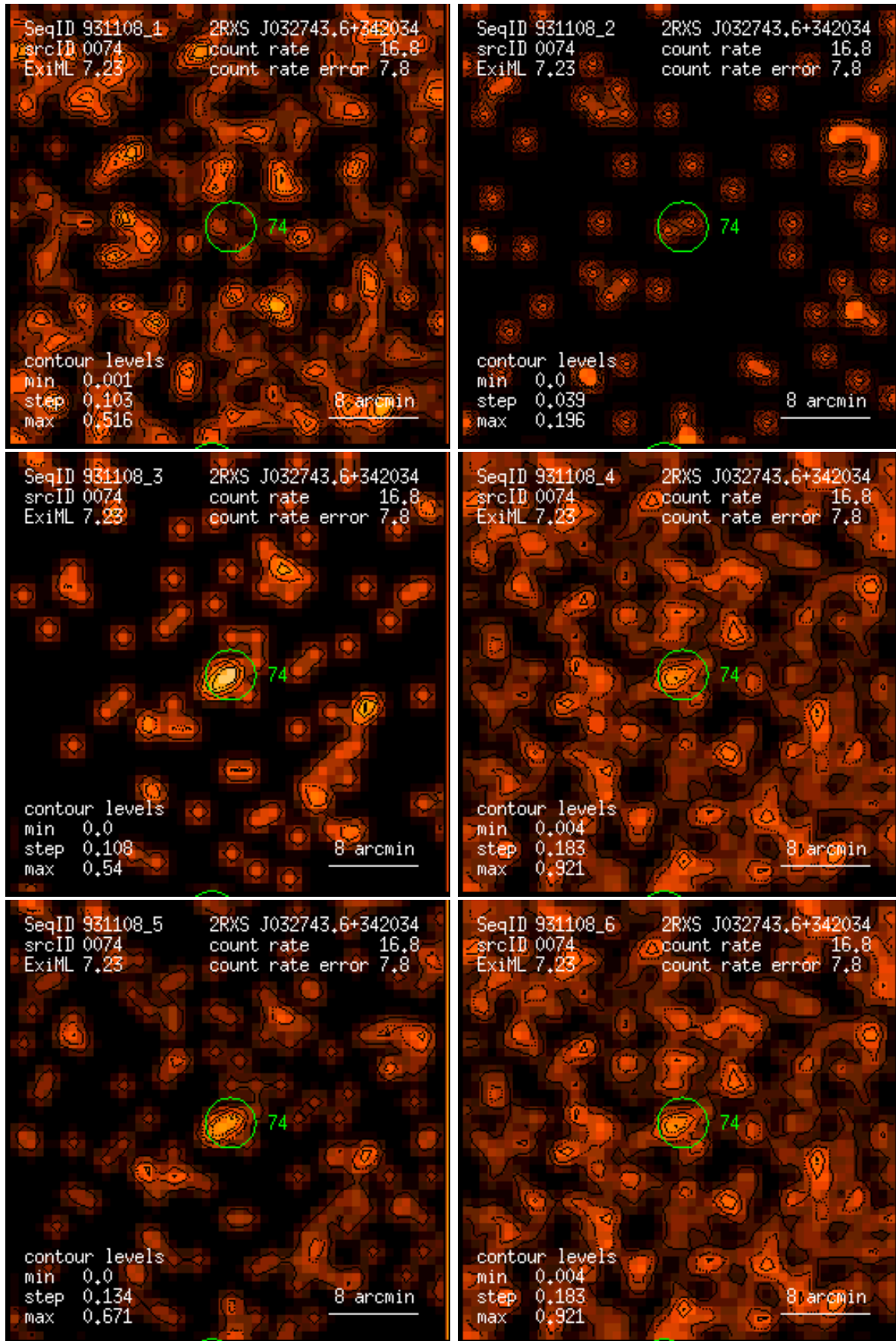
Figure 74: RASS 931108: detection 0074: band rate images, Gaussian filter: (1) PSPC channels 11 – 41, (2) 52 – 90, (3) 91 – 201, (4) 11 – 235, (5) 52 – 201, (6) 11 – 201. Broad band rates in counts/ks. Band rate contour levels in counts/ks/arcmin 2 .
