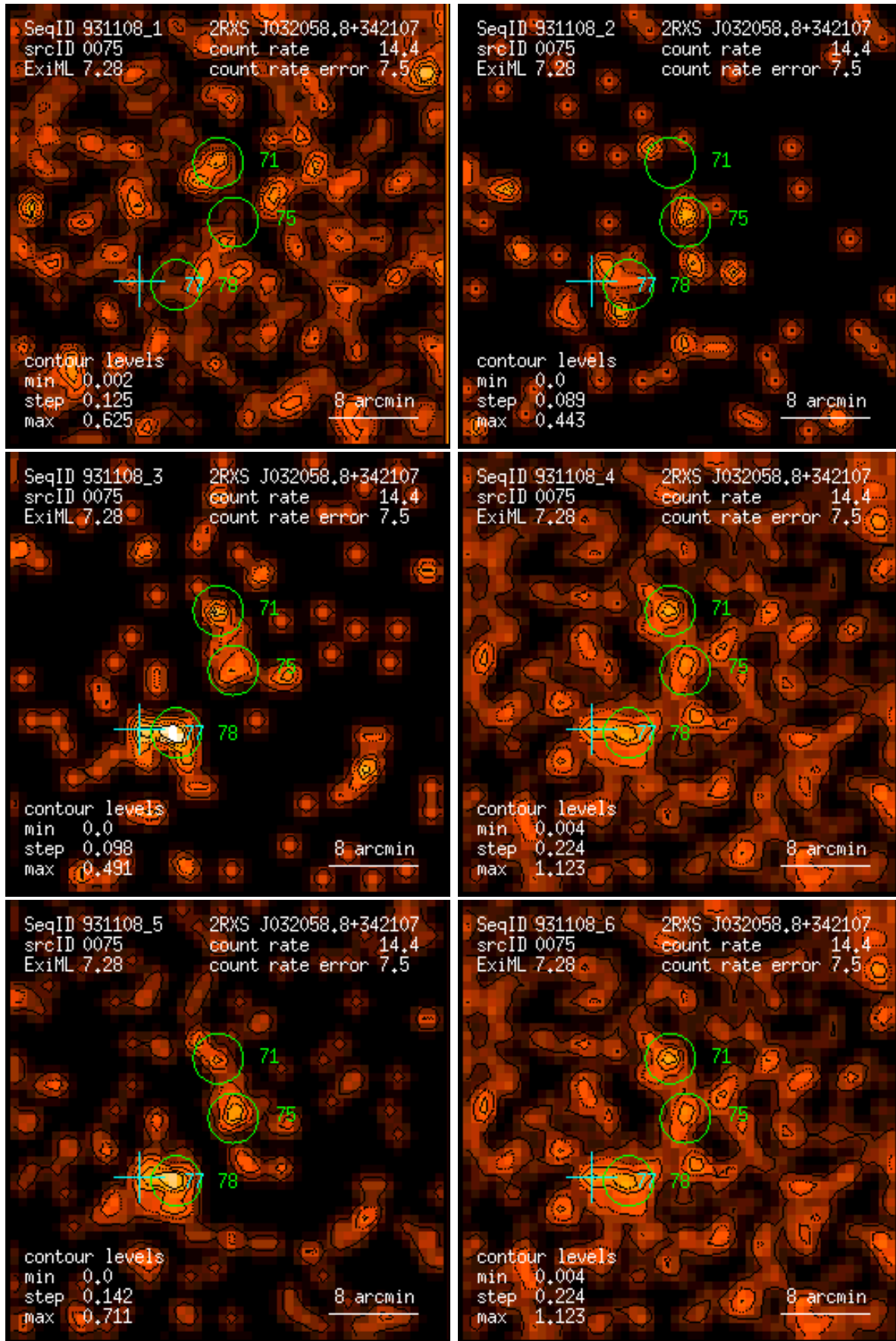
Figure 75: RASS 931108: detection 0075: band rate images, Gaussian filter: (1) PSPC channels 11 – 41, (2) 52 – 90, (3) 91 – 201, (4) 11 – 235, (5) 52 – 201, (6) 11 – 201. Broad band rates in counts/ks. Band rate contour levels in counts/ks/arcmin 2 .
