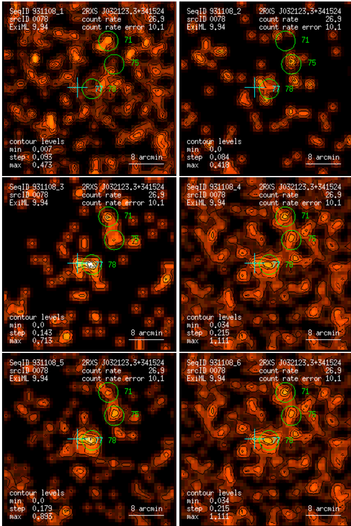
Figure 78: RASS 931108: detection 0078: band rate images, Gaussian filter: (1) PSPC channels 11 – 41, (2) 52 – 90, (3) 91 – 201, (4) 11 – 235, (5) 52 – 201, (6) 11 – 201. Broad band rates in counts/ks. Band rate contour levels in counts/ks/arcmin 2 .
