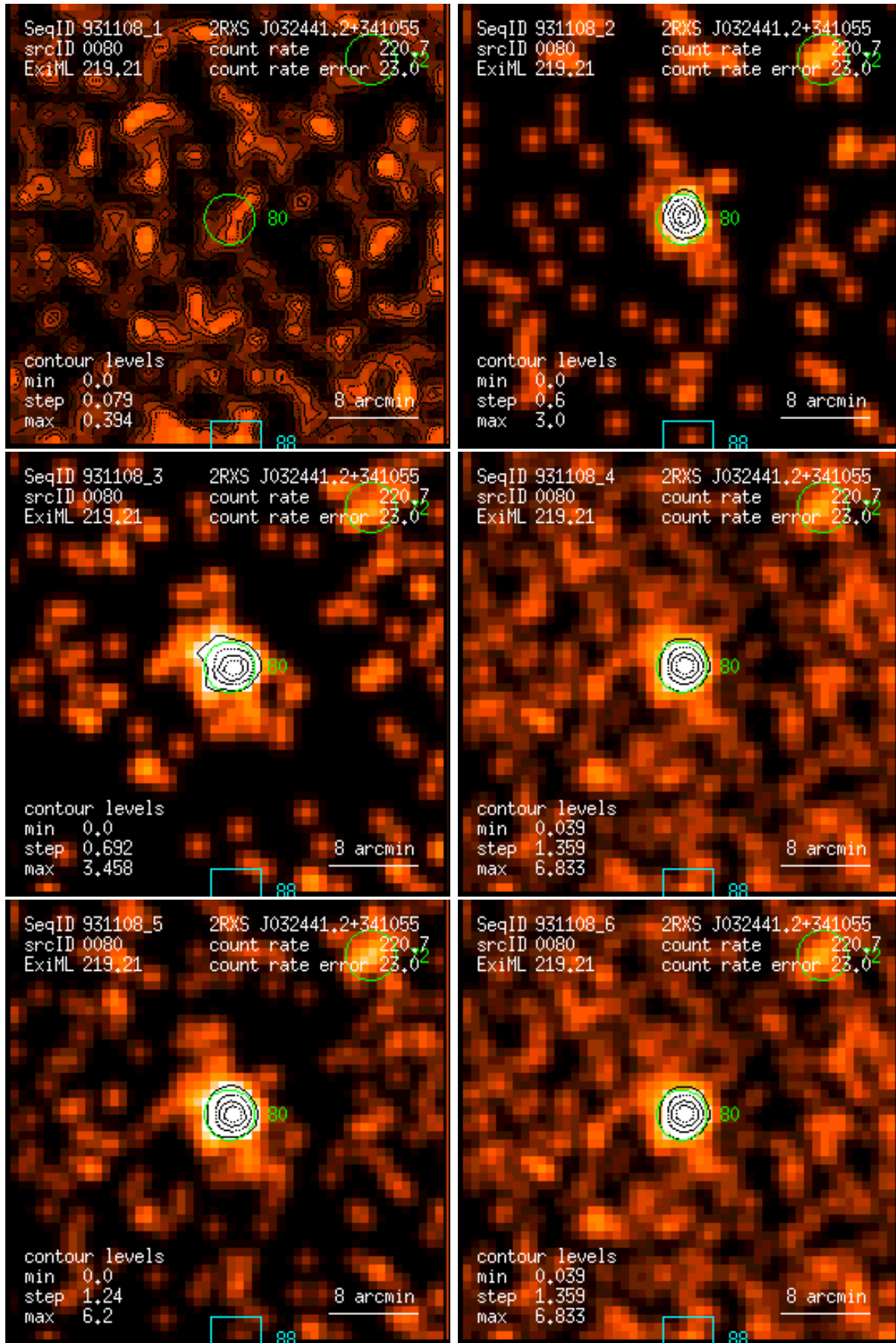
Figure 80: RASS 931108: detection 0080: band rate images, Gaussian filter: (1) PSPC channels 11 – 41, (2) 52 – 90, (3) 91 – 201, (4) 11 – 235, (5) 52 – 201, (6) 11 – 201. Broad band rates in counts/ks. Band rate contour levels in counts/ks/arcmin 2 .
