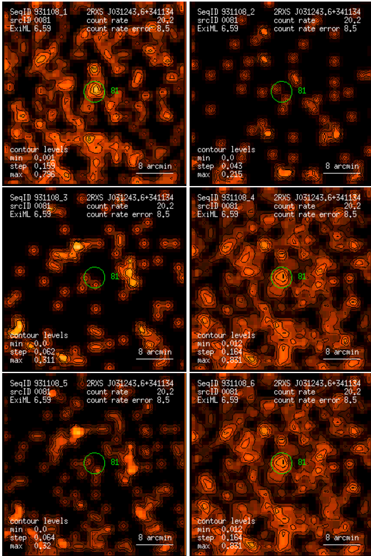
Figure 81: RASS 931108: detection 0081: band rate images, Gaussian filter: (1) PSPC channels 11 – 41, (2) 52 – 90, (3) 91 – 201, (4) 11 – 235, (5) 52 – 201, (6) 11 – 201. Broad band rates in counts/ks. Band rate contour levels in counts/ks/arcmin 2 .
