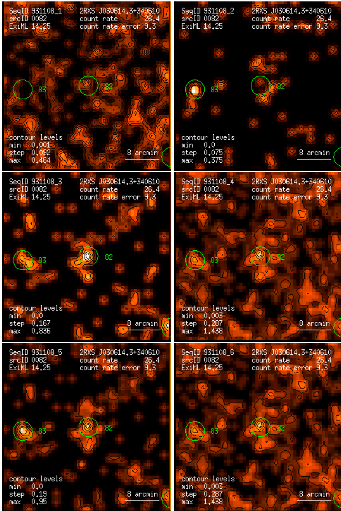
Figure 82: RASS 931108: detection 0082: band rate images, Gaussian filter: (1) PSPC channels 11 – 41, (2) 52 – 90, (3) 91 – 201, (4) 11 – 235, (5) 52 – 201, (6) 11 – 201. Broad band rates in counts/ks. Band rate contour levels in counts/ks/arcmin 2 .
