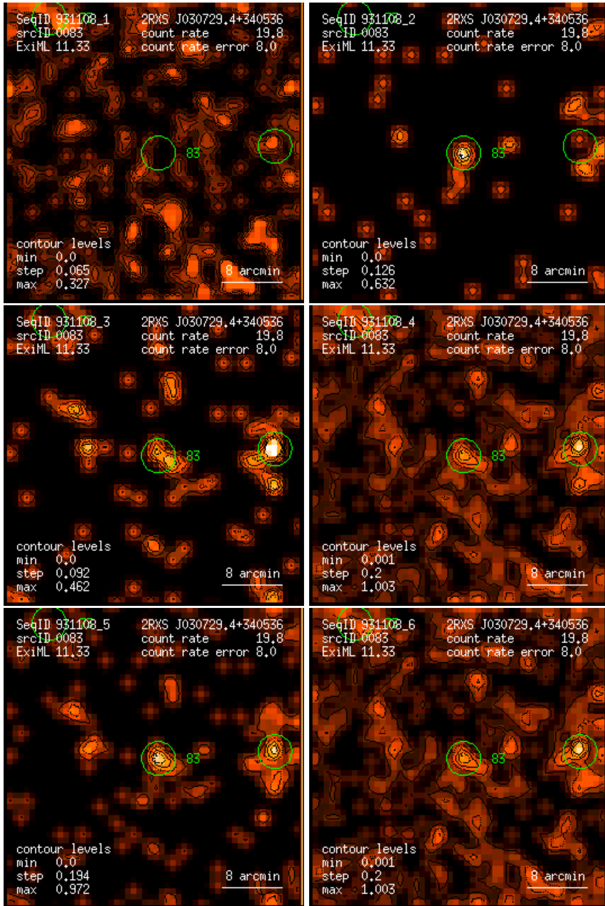
Figure 83: RASS 931108: detection 0083: band rate images, Gaussian filter: (1) PSPC channels 11 – 41, (2) 52 – 90, (3) 91 – 201, (4) 11 – 235, (5) 52 – 201, (6) 11 – 201. Broad band rates in counts/ks. Band rate contour levels in counts/ks/arcmin 2 .
