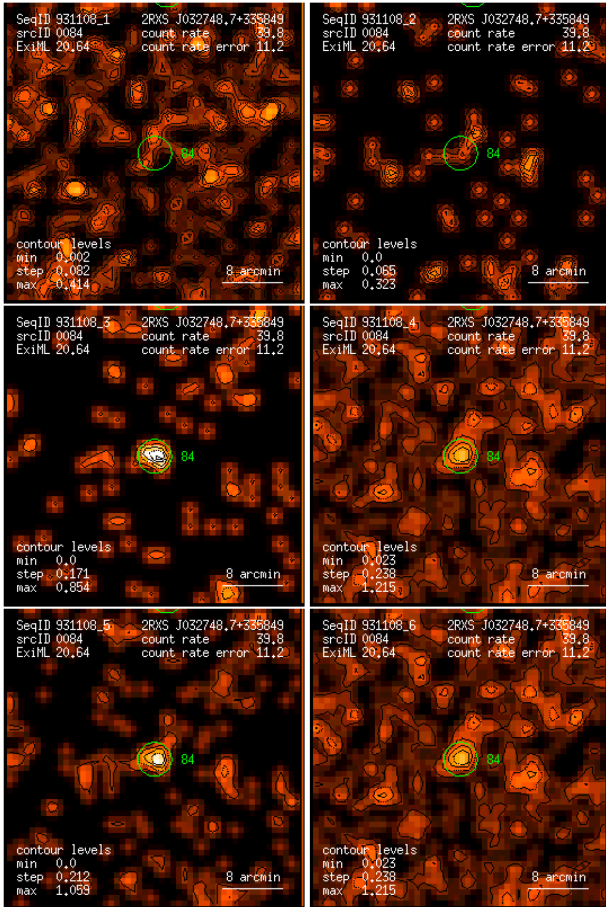
Figure 84: RASS 931108: detection 0084: band rate images, Gaussian filter: (1) PSPC channels 11 – 41, (2) 52 – 90, (3) 91 – 201, (4) 11 – 235, (5) 52 – 201, (6) 11 – 201. Broad band rates in counts/ks. Band rate contour levels in counts/ks/arcmin 2 .
