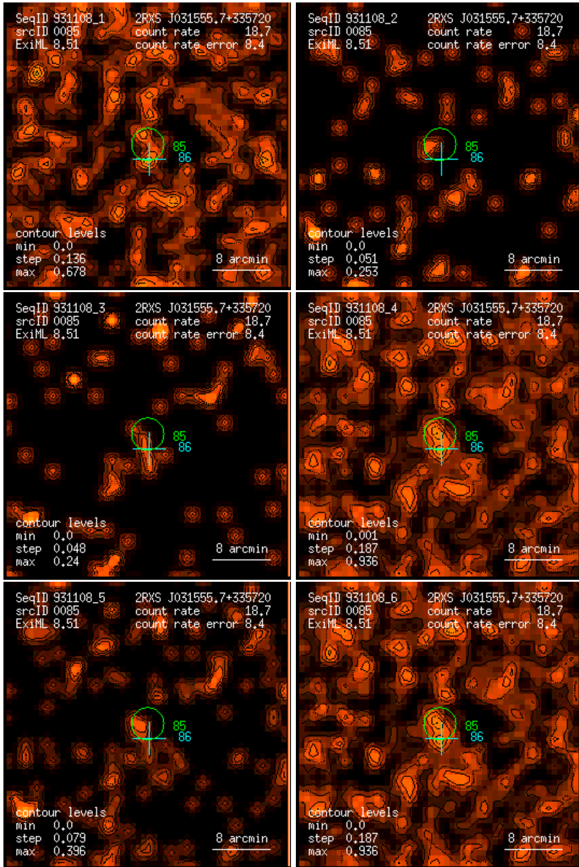
Figure 85: RASS 931108: detection 0085: band rate images, Gaussian filter: (1) PSPC channels 11 – 41, (2) 52 – 90, (3) 91 – 201, (4) 11 – 235, (5) 52 – 201, (6) 11 – 201. Broad band rates in counts/ks. Band rate contour levels in counts/ks/arcmin 2 .
