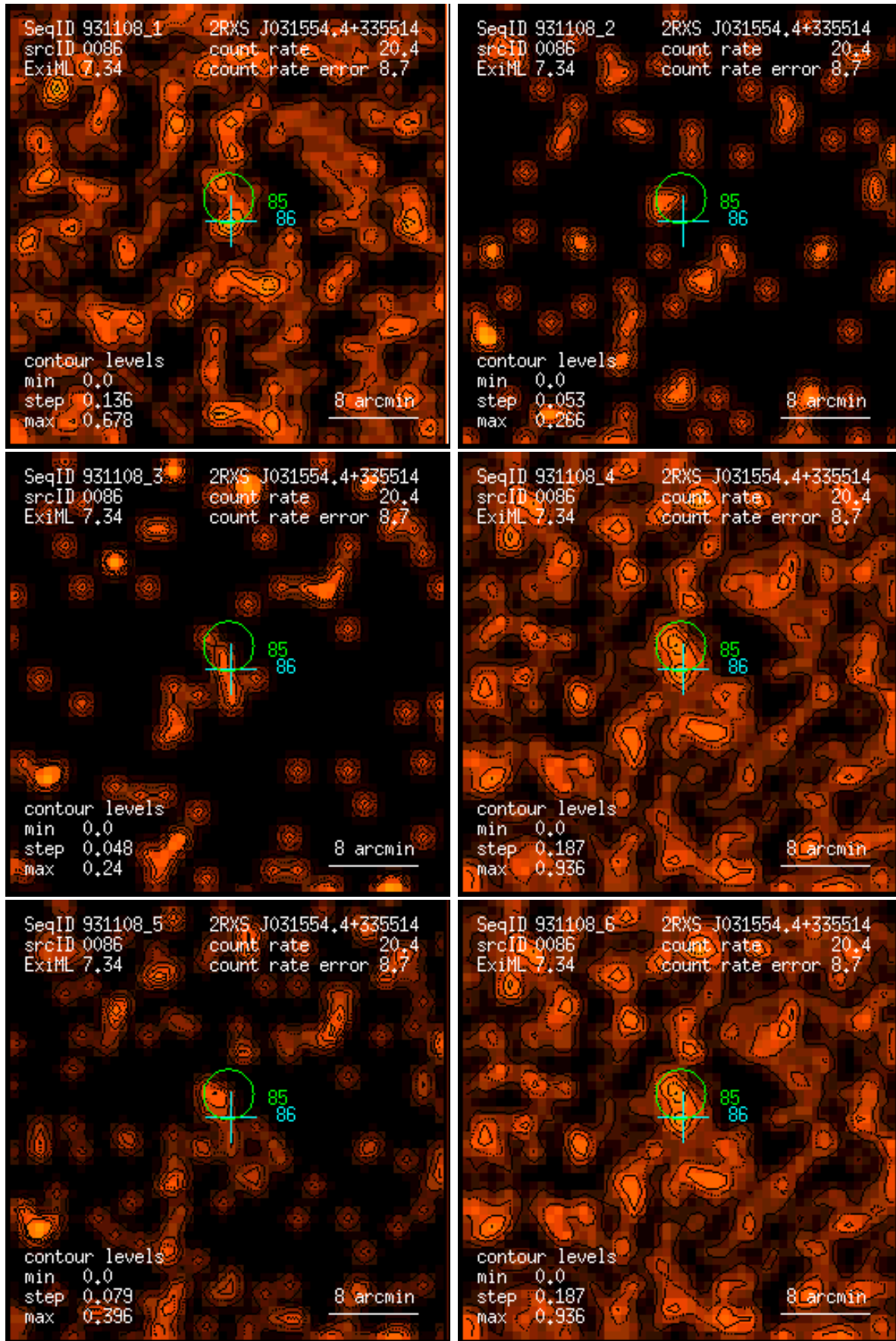
Figure 86: RASS 931108: detection 0086: band rate images, Gaussian filter: (1) PSPC channels 11 – 41, (2) 52 – 90, (3) 91 – 201, (4) 11 – 235, (5) 52 – 201, (6) 11 – 201. Broad band rates in counts/ks. Band rate contour levels in counts/ks/arcmin 2 .
