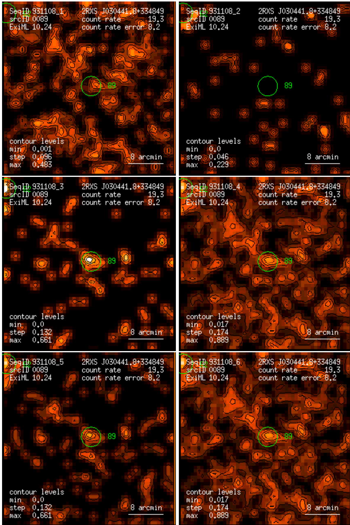
Figure 89: RASS 931108: detection 0089: band rate images, Gaussian filter: (1) PSPC channels 11 – 41, (2) 52 – 90, (3) 91 – 201, (4) 11 – 235, (5) 52 – 201, (6) 11 – 201. Broad band rates in counts/ks. Band rate contour levels in counts/ks/arcmin 2 .
