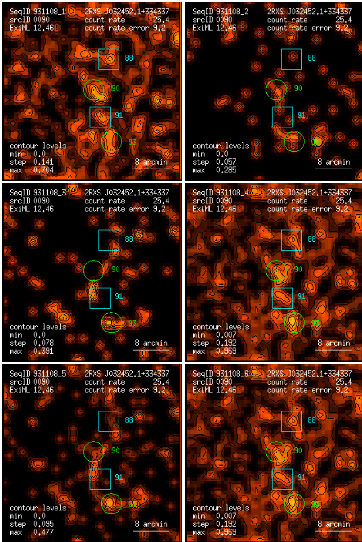
Figure 90: RASS 931108: detection 0090: band rate images, Gaussian filter: (1) PSPC channels 11 – 41, (2) 52 – 90, (3) 91 – 201, (4) 11 – 235, (5) 52 – 201, (6) 11 – 201. Broad band rates in counts/ks. Band rate contour levels in counts/ks/arcmin 2 .
