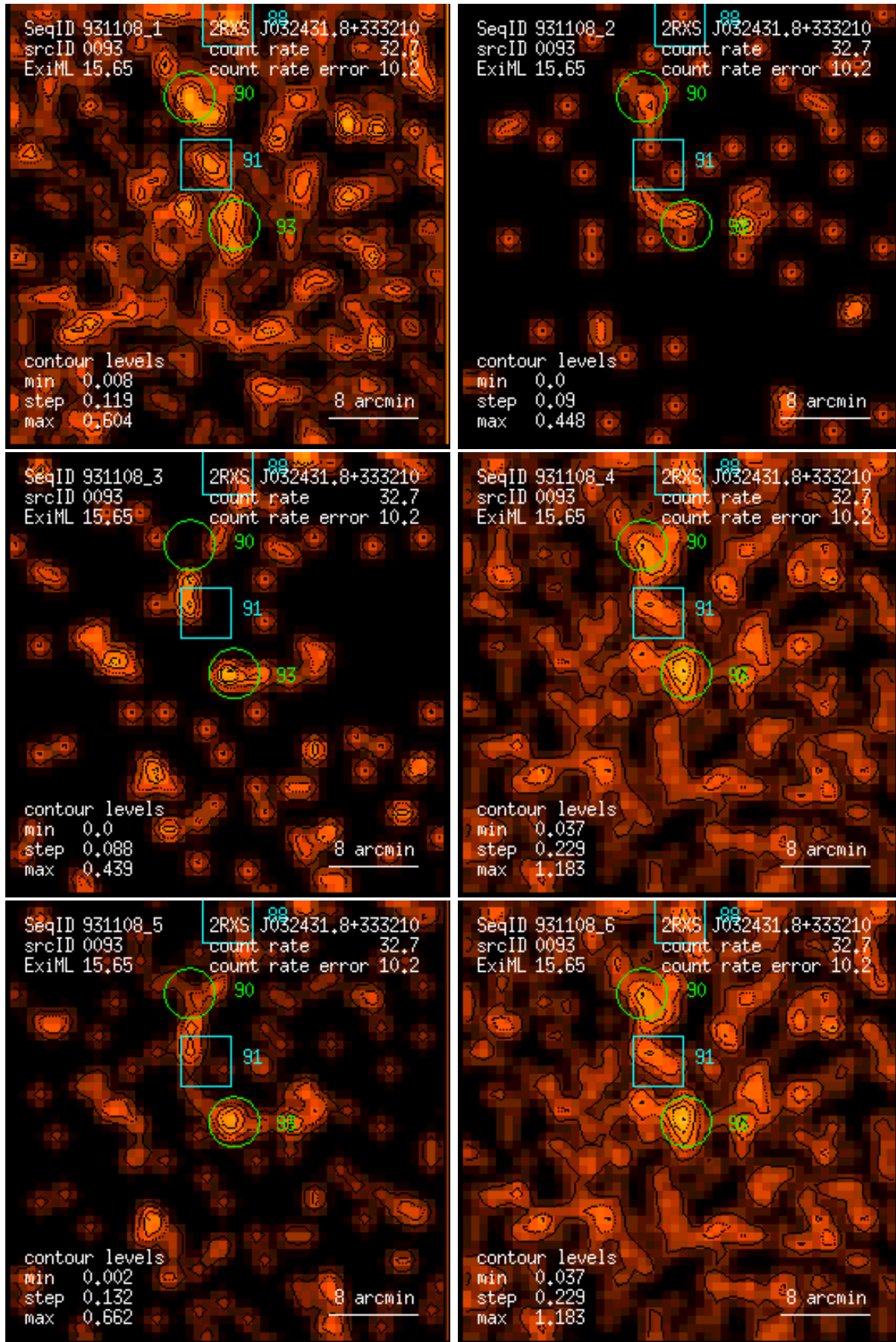
Figure 93: RASS 931108: detection 0093: band rate images, Gaussian filter: (1) PSPC channels 11 – 41, (2) 52 – 90, (3) 91 – 201, (4) 11 – 235, (5) 52 – 201, (6) 11 – 201. Broad band rates in counts/ks. Band rate contour levels in counts/ks/arcmin 2 .
