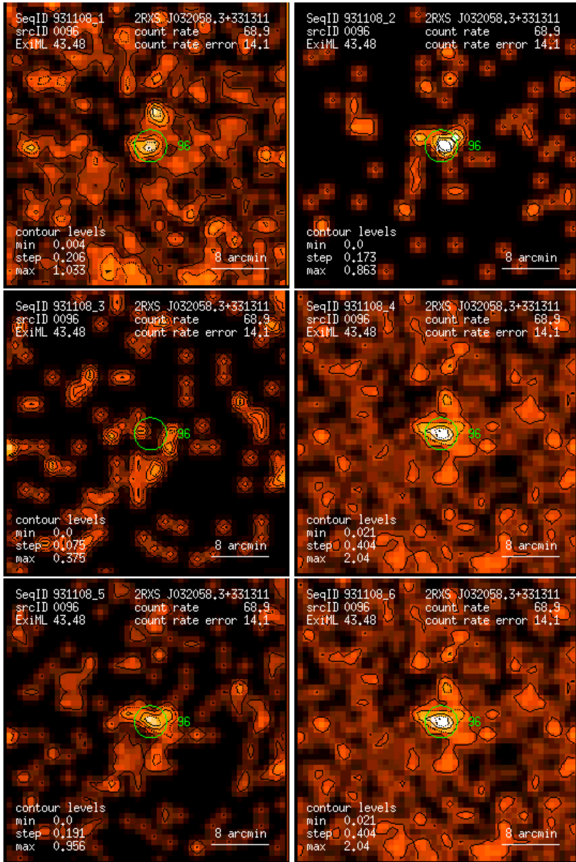
Figure 96: RASS 931108: detection 0096: band rate images, Gaussian filter: (1) PSPC channels 11 – 41, (2) 52 – 90, (3) 91 – 201, (4) 11 – 235, (5) 52 – 201, (6) 11 – 201. Broad band rates in counts/ks. Band rate contour levels in counts/ks/arcmin 2 .
