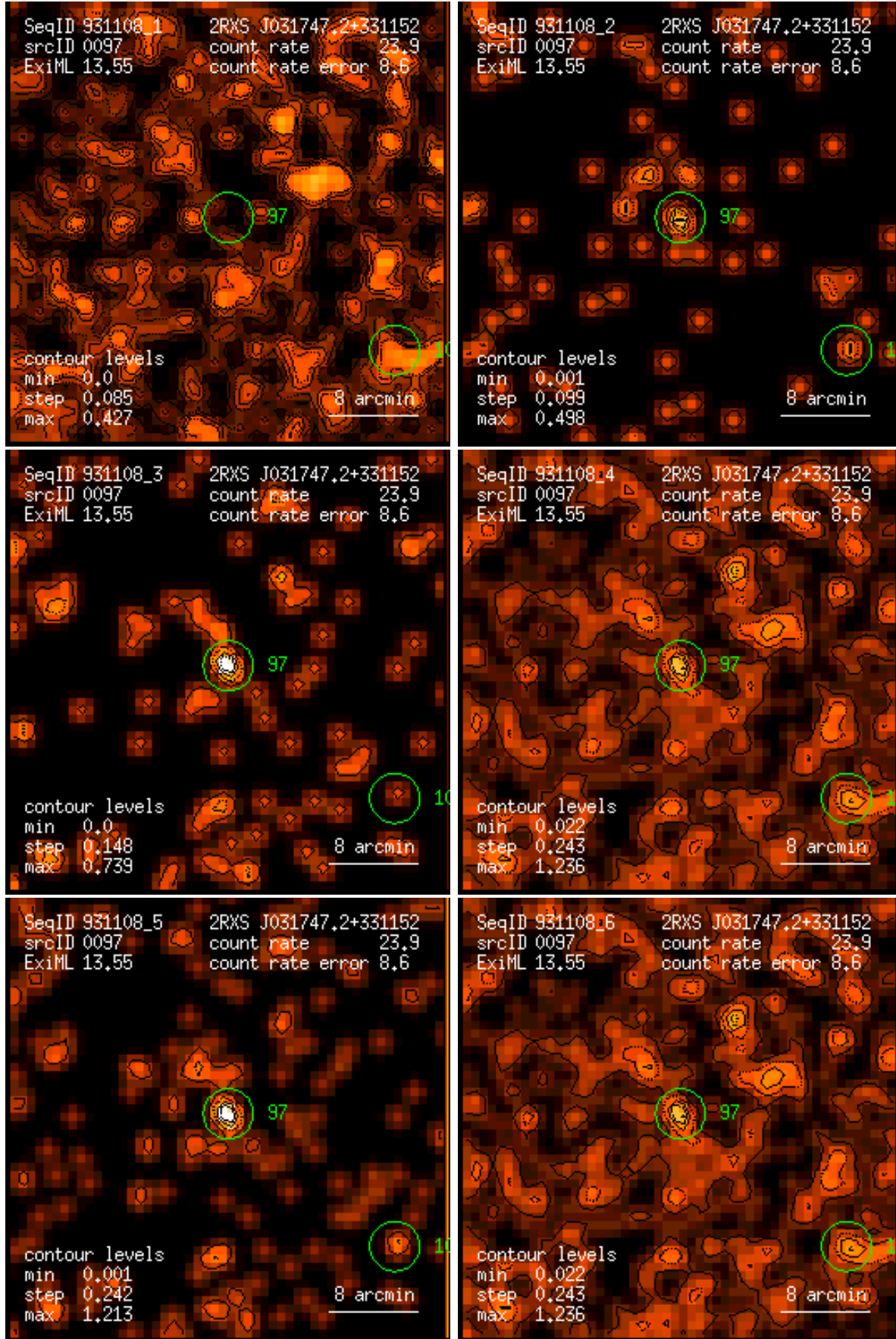
Figure 97: RASS 931108: detection 0097: band rate images, Gaussian filter: (1) PSPC channels 11 – 41, (2) 52 – 90, (3) 91 – 201, (4) 11 – 235, (5) 52 – 201, (6) 11 – 201. Broad band rates in counts/ks. Band rate contour levels in counts/ks/arcmin 2 .
