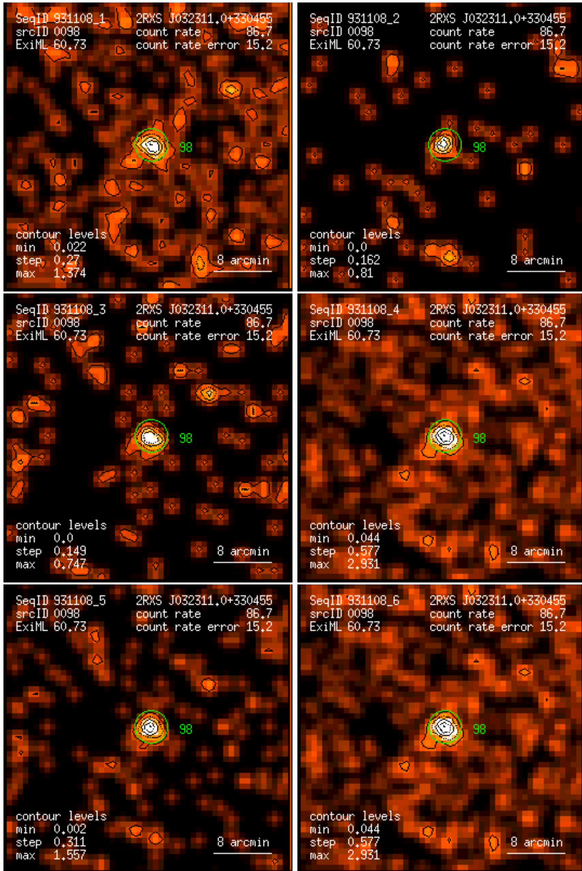
Figure 98: RASS 931108: detection 0098: band rate images, Gaussian filter: (1) PSPC channels 11 – 41, (2) 52 – 90, (3) 91 – 201, (4) 11 – 235, (5) 52 – 201, (6) 11 – 201. Broad band rates in counts/ks. Band rate contour levels in counts/ks/arcmin 2 .
